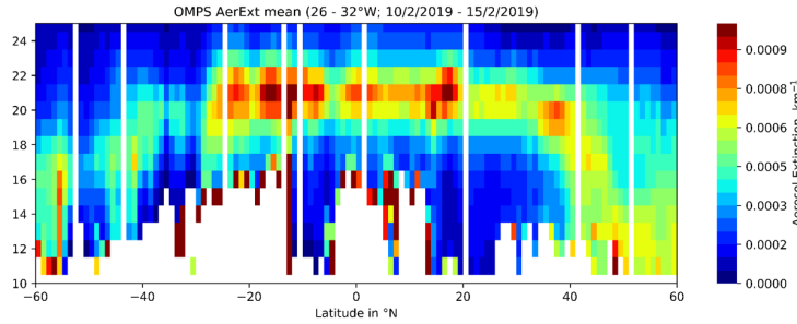
Figure 5. OMPS aerosol extinction data (at 675 nm) averaged for each 1° latitude bin between 10-15 th of Feb at 26-32°W.
