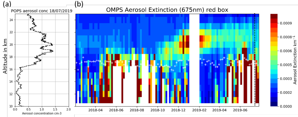
Figure 4. (a) In situ POPS aerosol concentration measurements at 17.5°N and 78.2°E, observed during the BATIAL campaign in 18/07/2019 for particle sizes from 0.15 to 0.18 μm. (b) OMPS aerosol extinction measurements (at 675 nm) averaged over 17-21°N, 76-82°E (location indicated with a small red area in Fig. 2) with 5-days averages. The point in time of the in situ profile from (a) is indicated with the black dotted line. White plus signs represent the mean tropopause altitude for the averaged profiles.
