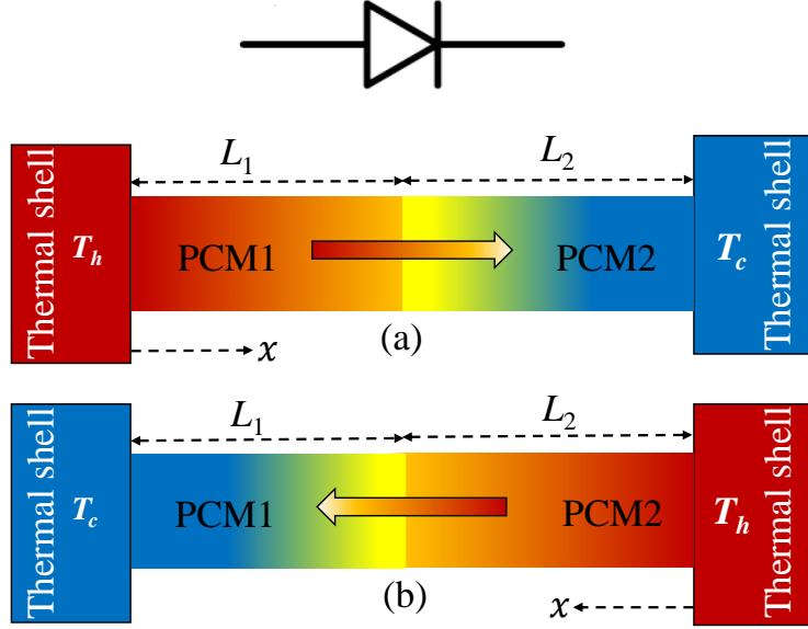
Figure 1: Scheme of a dual PCMs conductive thermal diode operating in the (a) forward and (b) backward configurations. Hot and cool thermal shells are set at the temperatures T_h and T_c , respectively.
