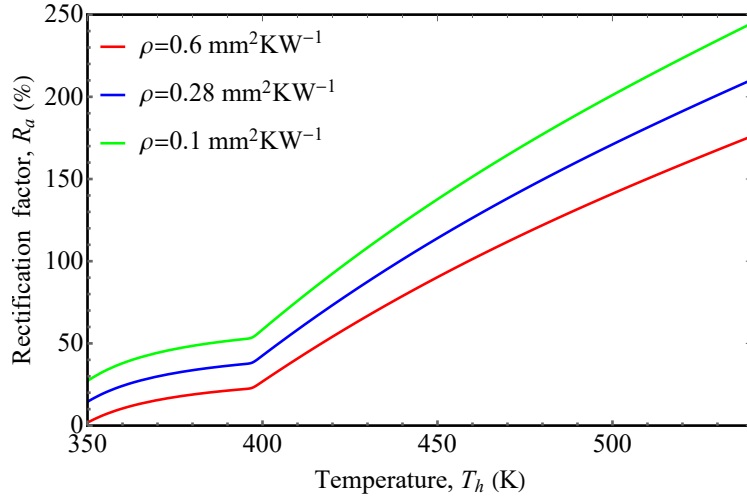
Figure 9: Rectification factor R of the conductive thermal diode as a function of the temperature T_h . Calculations were done by using the alternative definition R_a = [\max(q_F, q_B)/\min(q_F, q_B)] - 1 for three representative interface thermal resistances and T_c = 300 K.
