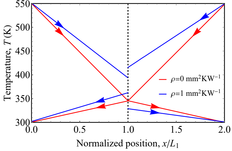
Figure 6: Temperature profiles within the terminals of the conductive thermal diode operating in the forward and backward configurations. Arrows stand for the direction of heat flux and calculations were done for T_c = 300 K, T_h = 550 K, and two values of the interface thermal resistance \rho .
