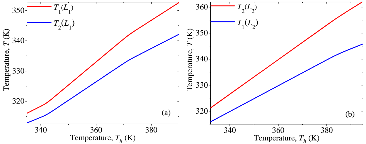
Figure 5: Interface temperatures for the (a) forward [ T_1(L_1) and T_2(L_1) ] and (b) backward [ T_2(L_2) and T_1(L_2) ] configurations, as functions of the temperature T_h . Calculations were done for T_c = 300 K and \rho = 1 mm 2 KW -1 .
