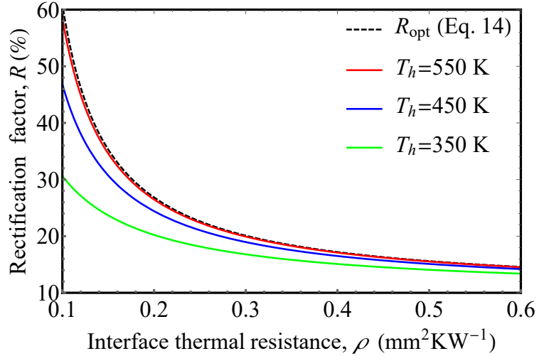
Figure 7: Rectification factor of the conductive thermal diode, as a function of the interface thermal resistance \rho . Calculations were done using R = [1 - \min(q_F, q_B)/\max(q_F, q_B)] and T_c = 300 K.
