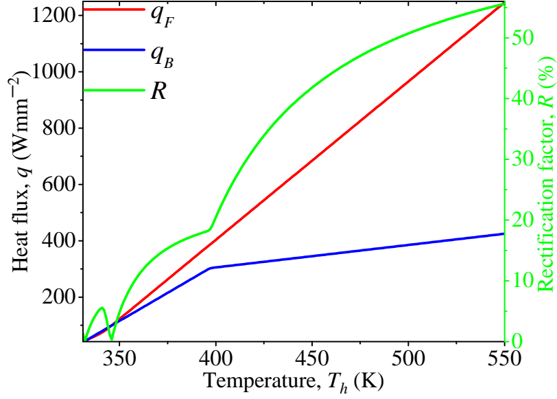
Figure 3: Rectification factor, forward and backward heat fluxes of the conductive thermal diode of VO 2 and PE, as functions of the temperature T_h . Calculations were done for T_c = 300 K and \rho = 0 \text{ mm}^2\text{KW}^{-1} .
