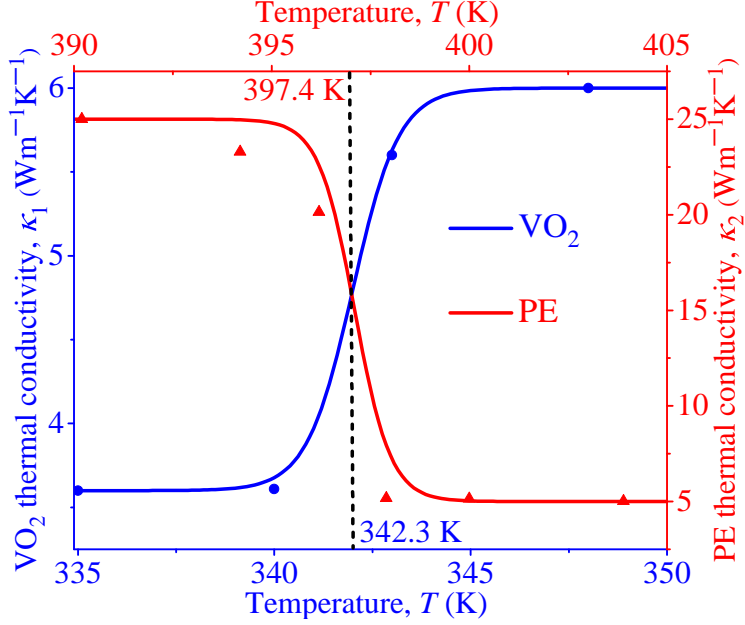
Figure 2: Thermal conductivities of VO 2 and PE, as functions of the temperature within their corresponding MIT. Dots and triangles stand for experimental data reported in the literature [37, 33], while lines represent the theoretical predictions of Eq. (3).
