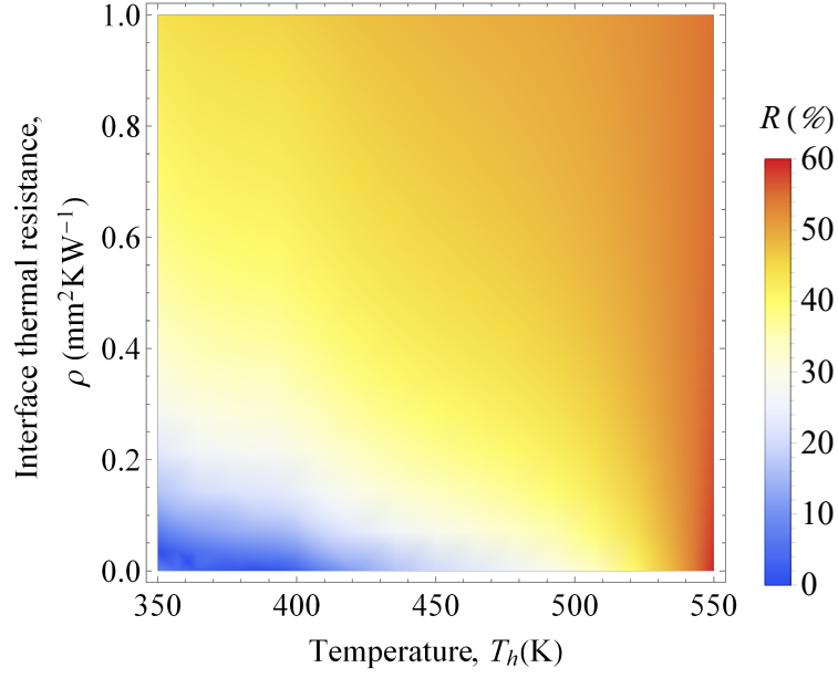
Figure 8: Density plot of the conductive thermal diode rectification factor as a function of the temperature T_h and interface thermal resistance \rho . Calculations were done using R = [1 - \min(q_F, q_B)/\max(q_F, q_B)] and T_c = 300 K.
