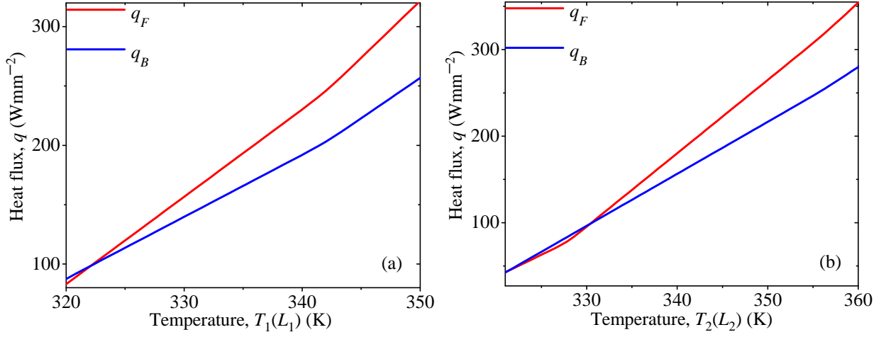
Figure 4: Temperature evolution of the forward and backward heat fluxes, as functions of (a) T_1(L_1) and (b) T_2(L_2) . Calculations were done for T_c = 300 K and \rho = 0 mm 2 KW -1 .
