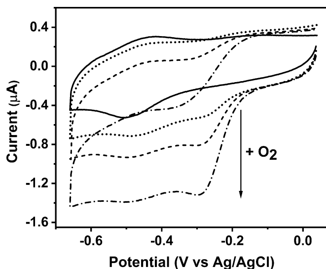
Figure 4. Cyclic voltammograms of the GRW-L16CL30H mini-heme protein (48 μM heme and 144 μM monomeric peptide concentrations) in 250 mM TRIS-maleate buffer at pH 10.1, entrapped in a thin layer at a pyrolytic graphite electrode, 20 mV s -1 scan rate. In strict anaerobic conditions, the well-defined redox peaks revealed a redox potential ( E_{1/2} ) at -460 mV vs. Ag/AgCl for the Fe III /Fe II redox couple (solid trace). In the presence of O 2 , the amplitude of the additional cathodic wave, with no anodic counterpart (dotted trace), was proportional to the increase in O 2 concentrations (see arrow), reflecting the catalytic reduction of dioxygen by the mini-heme protein. Experimental conditions as in Figure S8.
