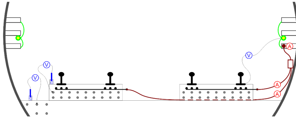
Figure 1. Sketch of ETS tunnel section subject to verification of stray current and corrosion potential: running rails and SCD rebars (black), other reinforcement (gray), connecting cables and SCC (brown), earthing equipotential conductor (yellow/green), voltmetric measurements and half-cells for concrete potential reading (blue), and amperometric measurements (red)
