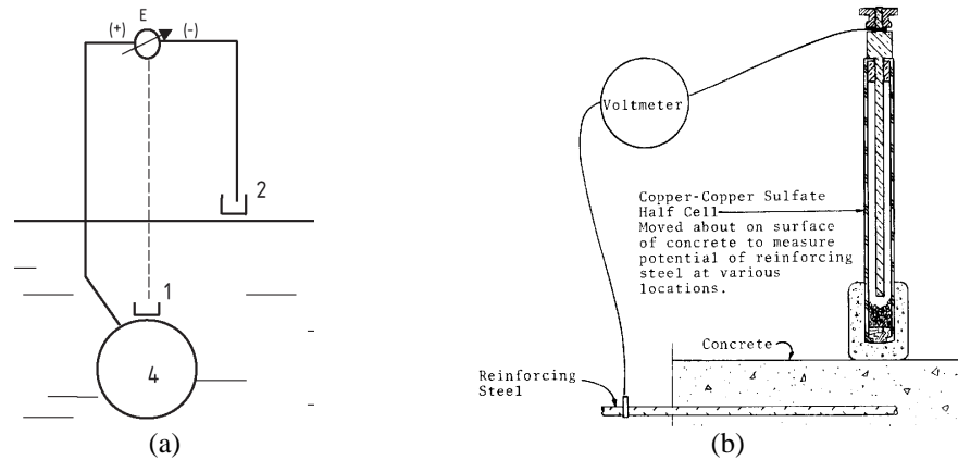
Figure 2. Potential measurements; (a) Pipe or buried structure, (b) Reinforcement rebar in concrete
