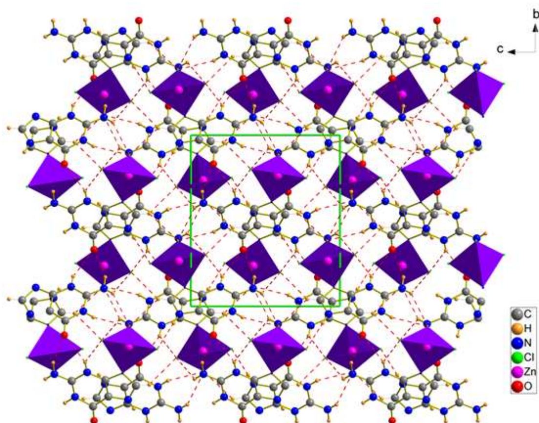
Fig. 2 A projection of the structure of [ZnCl 3 (C 5 H 6 N 5 O)] along the a -axis. Dotted lines indicate hydrogen bonds.
