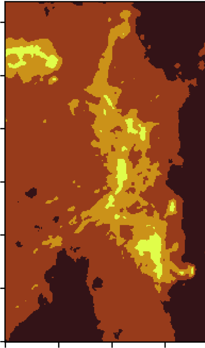
Fig. 13. Spatial distribution of the four following masks: 1 \leq A_v < 2 in black, 2 \leq A_v < 6 in brown, 6 \leq A_v < 15 in orange, and 15 \leq A_v in yellow.
