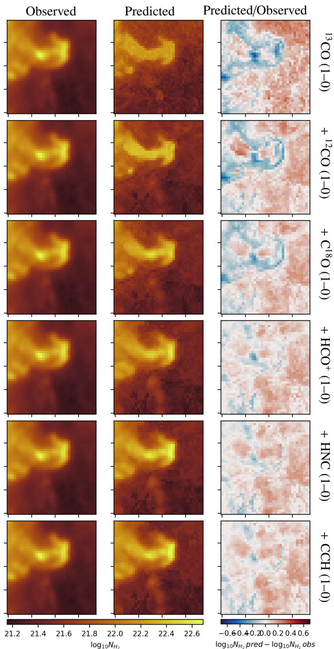
Fig. 11. Evolution of the prediction of the column density when adding molecular tracers one by one during the training phase. Left and middle columns: Spatial distribution of the observed and predicted column densities. Both images share the same color scale. Right column: Ratio of the predicted column density over the observed one. The limits of the color scale correspond to a ratio interval from 1/5 to 5.
