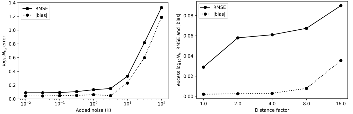
Fig. 16. Evolution of the accuracy (RMSE and mean error) of the \log(N_{\text{H}_2}/\text{cm}^{-2}) predictor when changing the condition of observations. Left: Gaussian noise of zero mean and a given standard deviation is added to the line spectrum. The median noises belong to the [0.03 and 0.11 K] interval depending on the line. Right: The line emission maps are smoothed in order to simulate an observation at a distance between 0.4 and 12.8 kpc.
