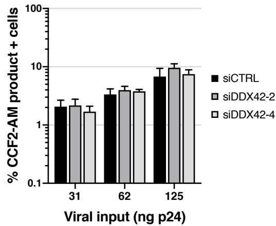
Supplementary Information Figure 7. DDX42 depletion does not affect HIV-1 entry. DDX42-depleted U87-MG/CD4/CXCR4 cells were infected with the indicated amounts of viruses carrying the \beta -lactamase (BlaM)-Vpr fusion protein for 3 hours. The cells were subsequently loaded with CCF2-AM substrate dye for 2h, washed extensively and incubated for another 16h for the reaction to develop. Cells positive for the CCF2-AM product were scored by flow cytometry. Data represent the mean \pm S.E.M of three independent experiments.
