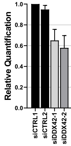
Supplementary Information Figure 4. DDX42 silencing efficiency in monocyte-derived macrophages. siRNA-transfected MDMs were harvested 48h post-transfection for RNA extraction and quantification of DDX42 mRNA levels by RT-qPCR. Actin and GAPDH were used as endogenous controls. Data represent the mean \pm S.E.M of three independent experiments performed with cells from 3 different blood donors.
