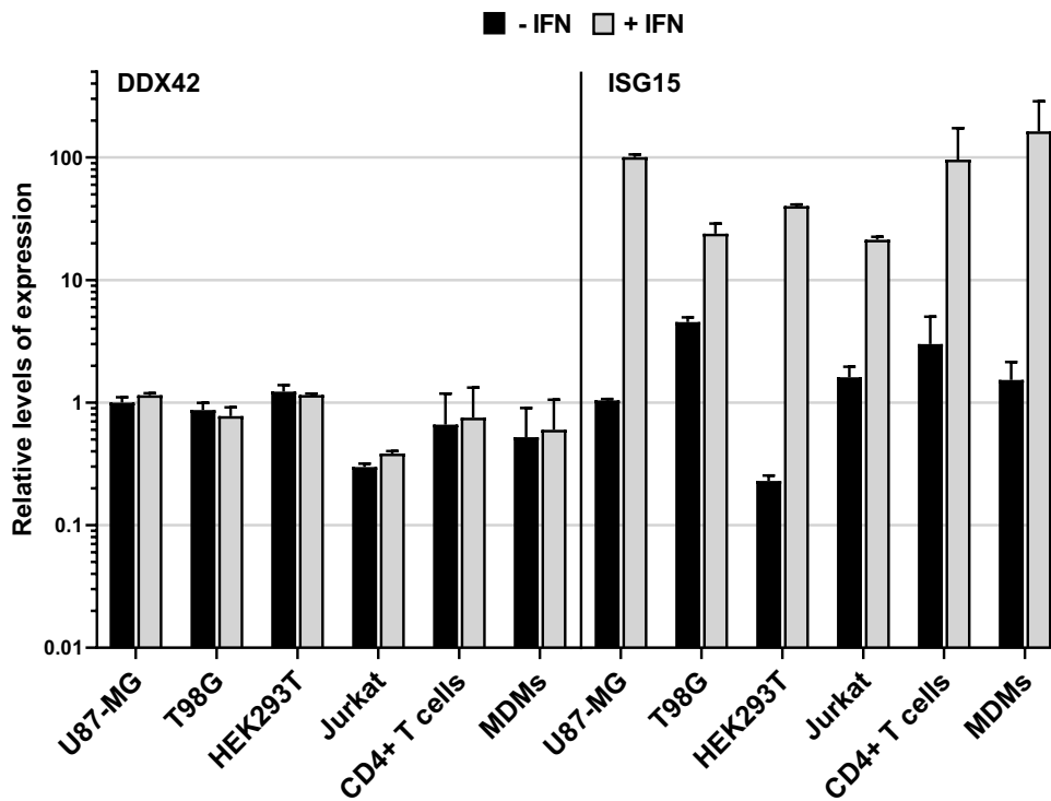
Supplementary Information Figure 3. DDX42 is not an ISG. The indicated primary cells or immortalized cell cultures were treated with IFN for 24 h or left untreated. RNA was subsequently extracted and DDX42 and ISG15 (a prototype ISG) mRNA levels were quantified by RT-qPCR; Actin B and GAPDH were used as endogenous controls. The bar chart shows the relative levels of expression of DDX42 and ISG15 in the presence or absence of IFN treatment. Data represent the mean \pm S.E.M of three independent experiments.
