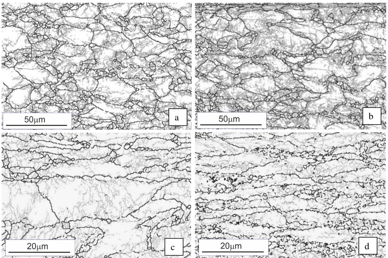
Fig. 3. Maps of the grain boundaries of low-carbon steel wire samples (longitudinal section), obtained by the classical technique ( a,c ) and by the experimental technique ( b,d ); \varnothing 5.0\text{mm} - ( a,b ); \varnothing 3.9 . HAGBs and LAGBs are marked black and grey respectively.
