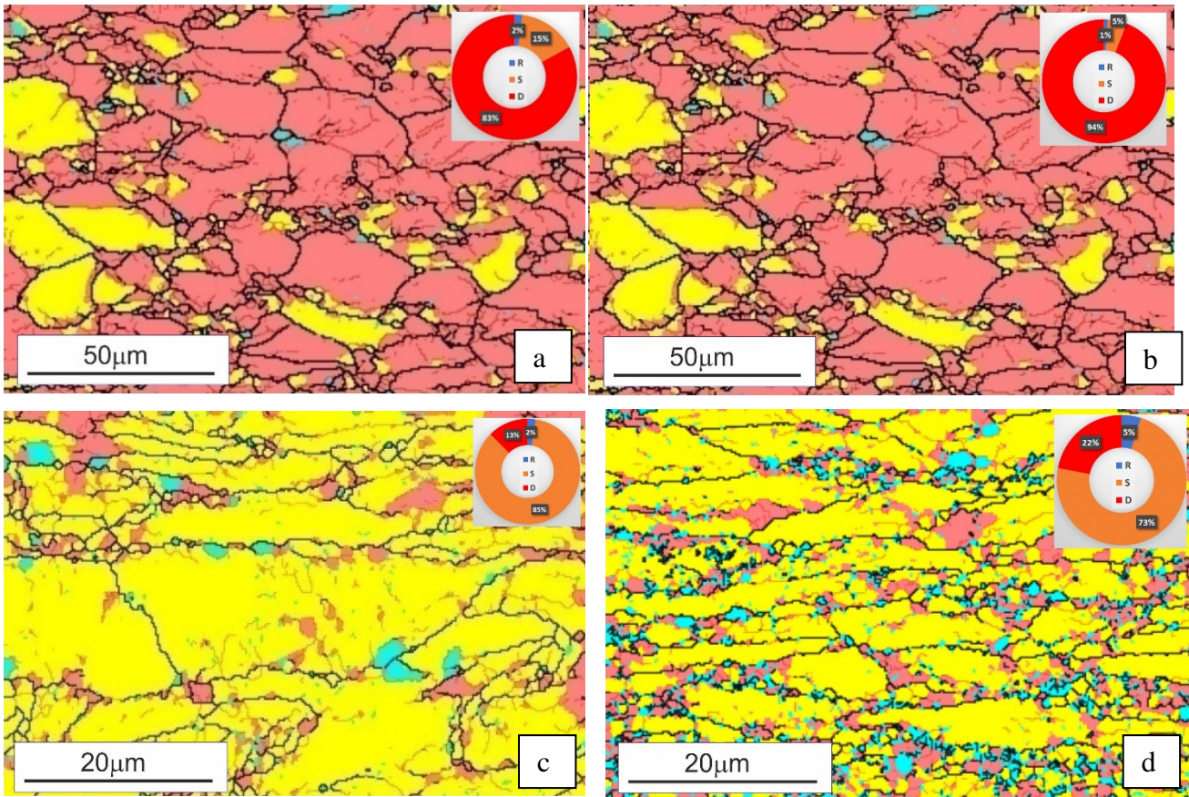
Fig. 5. Maps of the grain types in the samples of low-carbon steel wire samples (longitudinal section), obtained by the classical technique (a,c) and by the experimental technique (b,d); \varnothing 5.0\text{mm} - (a,b); \varnothing 3.9 - (c,d). The deformed (D), substructural (S) and recrystallized (R) grains are marked pink, yellow and blue, respectively
