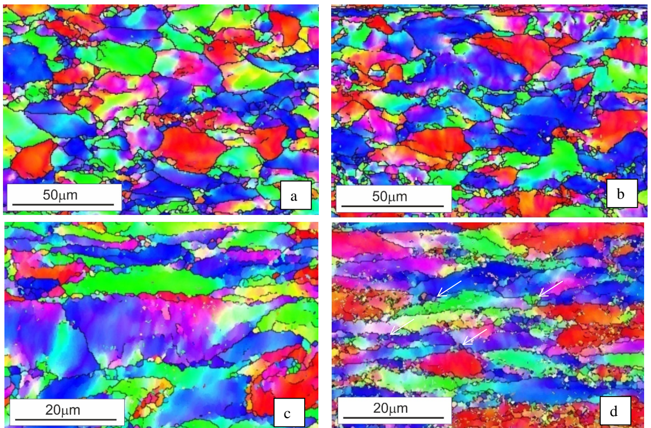
Fig. 4. IPF Maps of the crystallographic orientations of low-carbon steel wire samples (longitudinal section), obtained by the classical technique (a,c) and by the experimental technique (b,d); \varnothing 5.0\text{mm} - (a,b); \varnothing 3.9 - (c,d)
