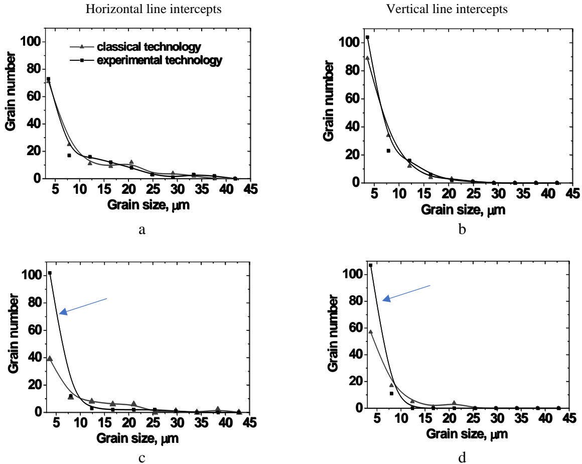
Fig. 2. Grain size histograms in the samples of the low-carbon steel wire. ; \text{Ø}5.0\text{mm} - (a, b) ; \text{Ø}3.9 - (c, d).
