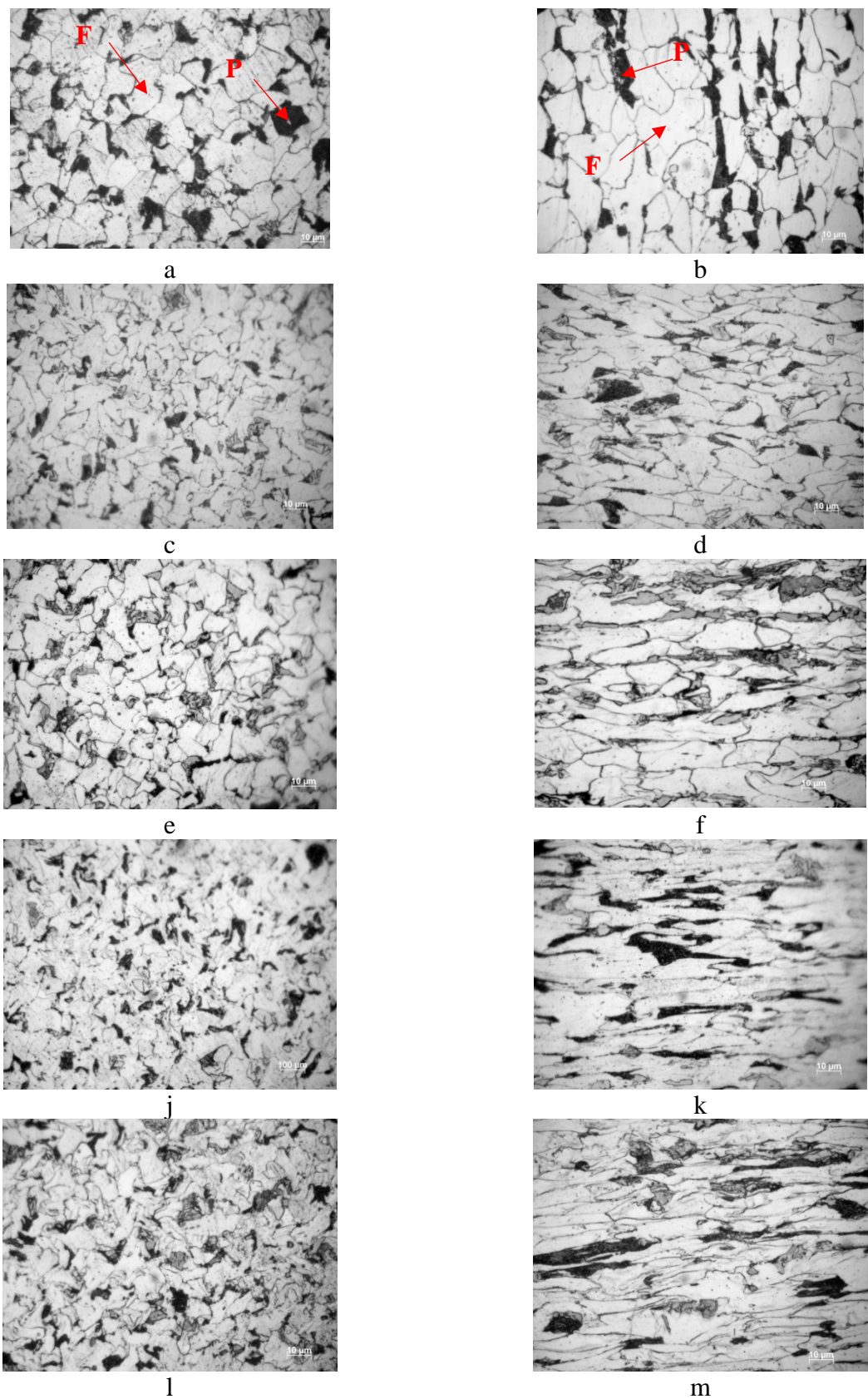
Fig.1. Microstructure of low-carbon steel wire after drawing: initial as received state (a,b), Ø6.15; classical technology (c,d,j,k); experimental technology (e,f,l,m); Ø5.0 - (c,d,e,f); Ø3.9 - (j,k,l,m); cross section - (a,c,e,j,l), longitudinal section - (b,d,f,k,m); magnification – x1000.
