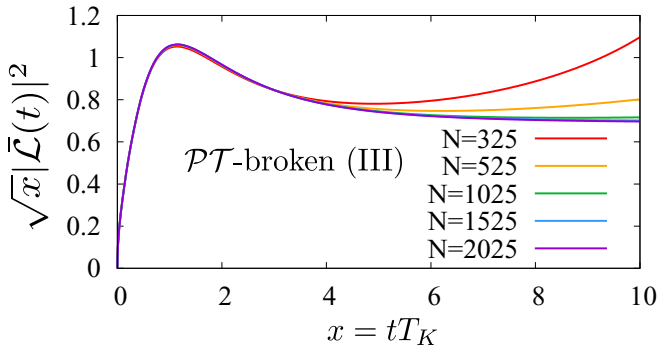
FIG. 11. Rescaled Loschmidt echo as a function of rescaled time for imaginary coupling \gamma = 0.2e^{i\pi/2} . Scaling factor T_K = |E_b^{\text{im}}| Eq. (23). Color labels different values of a system size.
