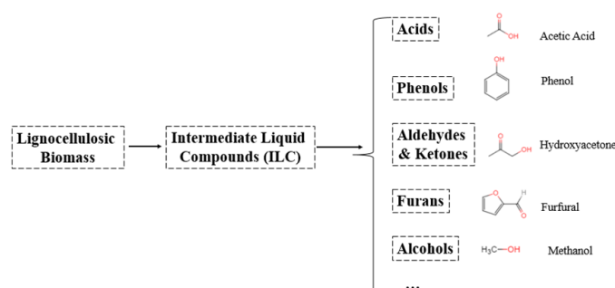
Figure 1. Proposed degradation model for lignocellulose pyrolysis
