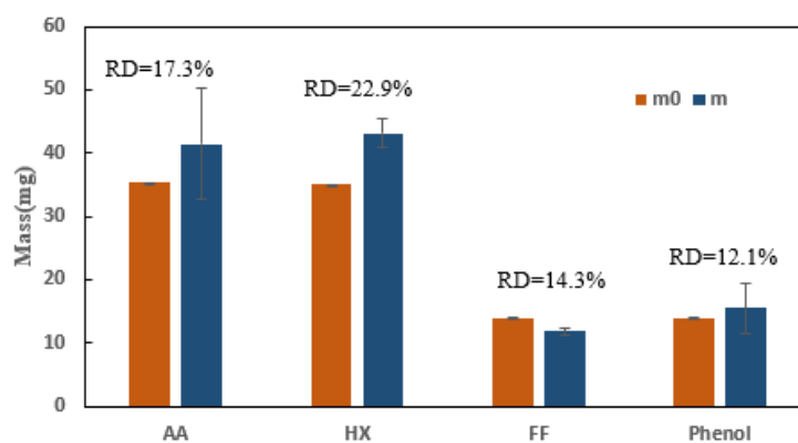
Figure 5. Mass balance for each analyte before ( m_0 ) and after ( m ) incubation at 90°C.
