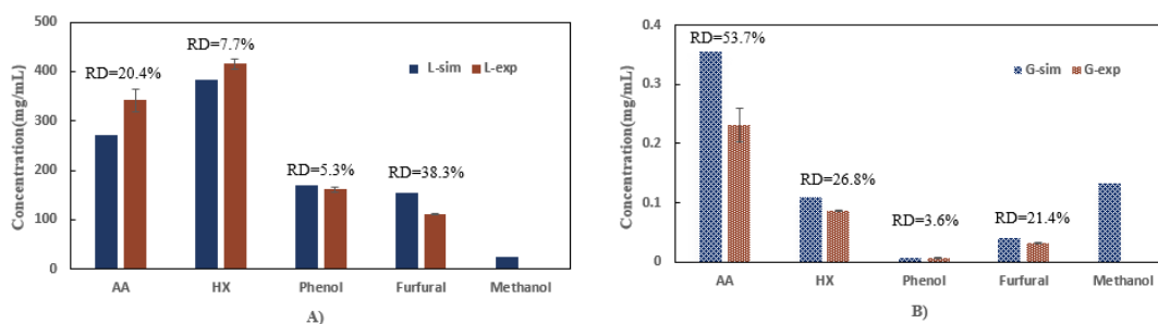
Figure 4. Concentrations of each component in ILC model mixture: A) in liquid phase and B) in vapour phase after an incubation period of 15 min at 90°C.
