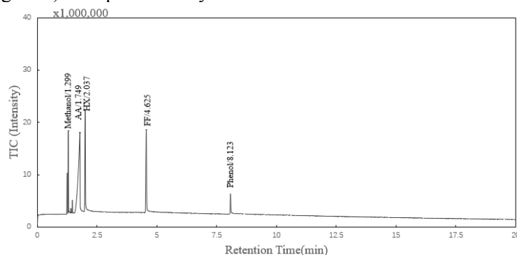
Figure 3. Chromatogram indicating the separation of each ILC model compound after incubation of 15 min at 90°C.
