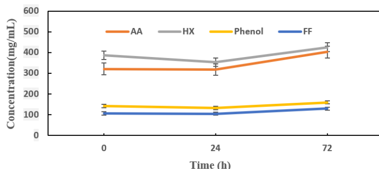
Figure 2. Concentrations measured in liquid mixture at 25°C before heating.
