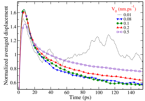
FIG. 8. Normalized averaged displacements \langle X_u(t) \rangle / V_0 for a set of increasing velocities 0.01 and 0.08, ..., 0.5 \text{nm.ps}^{-1} .
