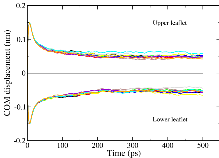
FIG. S1. Ten different bootstrap realizations of the displacement \langle x_u \rangle(t) for an initial kick impulsion V_0 = 0.09 \text{ nm}\cdot\text{ps}^{-1} .
