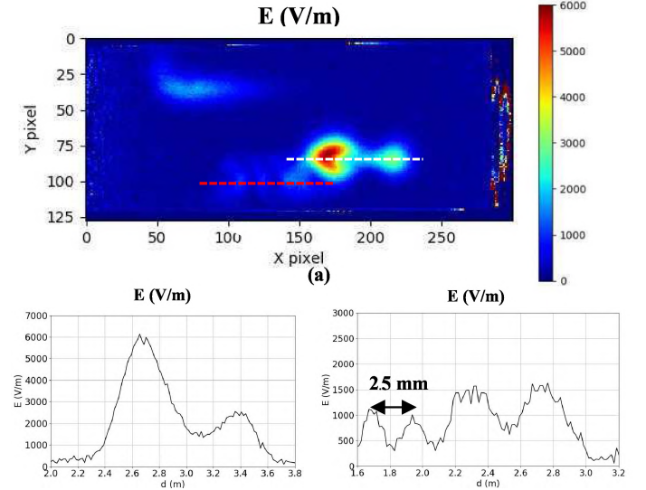
Figure 5 (a) Image of electric field of ZOR antenna at 4.29 GHz, (b) profile of the main lobe (white dotted), (c) profile of the secondary lobes (red dotted)
