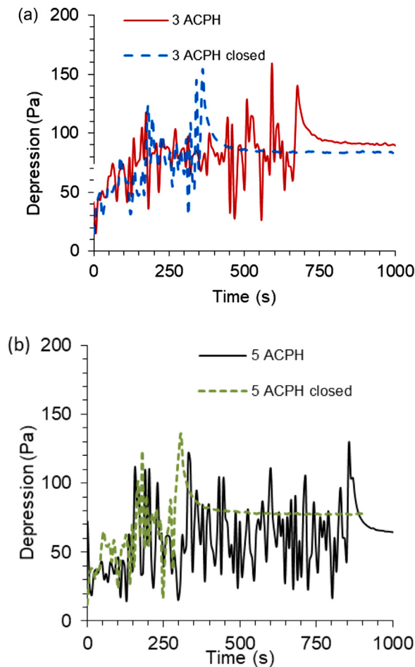
Fig. 4. Pressure as a function of time at the entrance of the exhaust duct (i.e. at the exit of the compartment) for heptane fires (pan diameter 0.3 m) at 3 (a) and 5 (b) ACPH (intake duct closed and opened).
