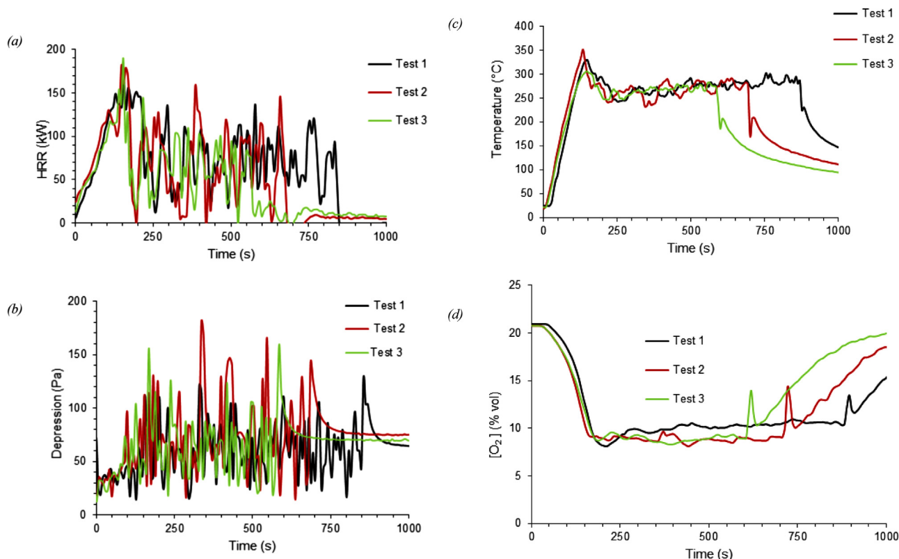
Fig. 2. Repeatability of heptane fires for a pan diameter of 0.3 m at 5 ACPH, intake duct open: (a) Heat Release Rates, (b) Depression, (c) Temperature, (d) Oxygen concentration.
