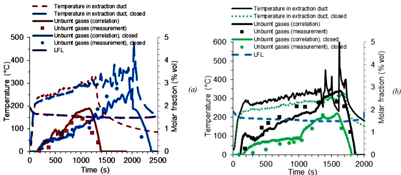
Fig. 14. Risk assessment of unburnt gas ignition at the entrance of the extraction duct. Dodecane fires, pan diameter of 0.4 m, opened and closed intake duct, (a) 3 ACPH and (b) 5 ACPH.
