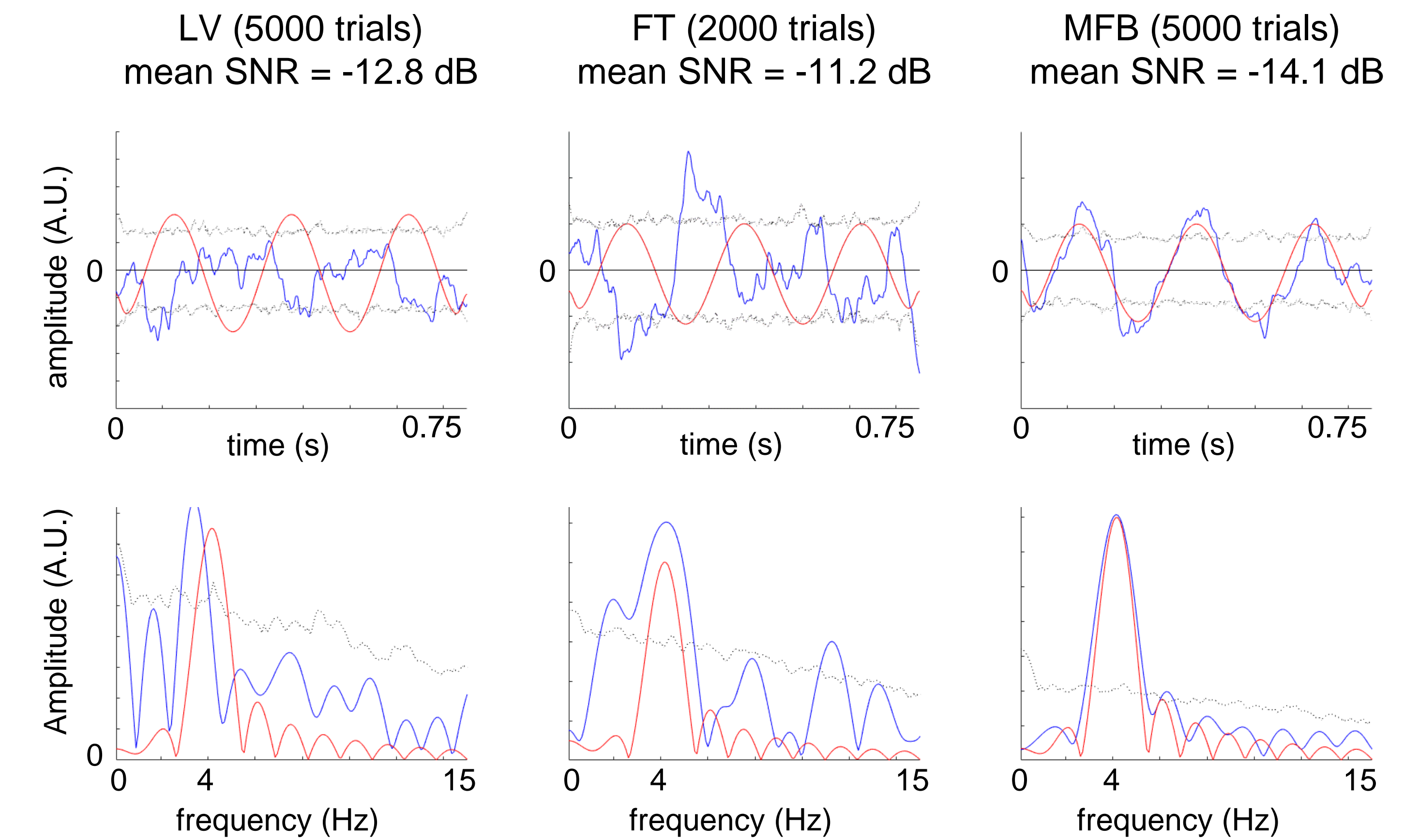
Blue lines: estimated psychophysical kernels for human (LV, FT) and simulated (MFB) participants, in the envelope (top) and Fourier (bottom) domains. Red lines: ideal template for the task. Dotted lines: 99% confidence interval under null hypothesis (permutation test).
