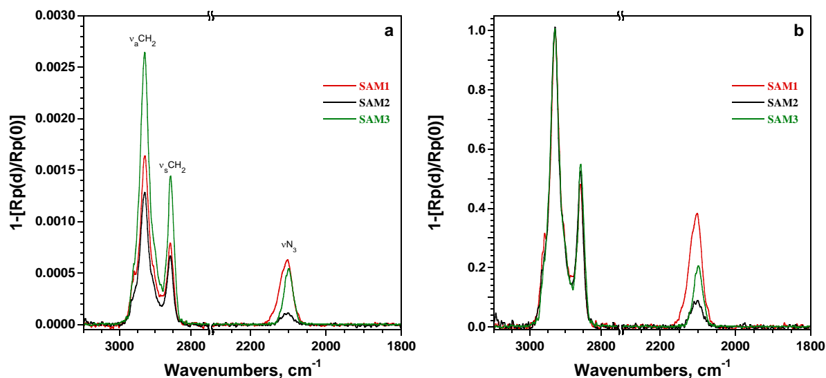
Figure 1. a) Non normalized and b) normalized PM-IRRAS spectra of SAM-N3 grafted onto \text{SiO}_2/\text{Au} substrate depending on the deposition processes in the 3100\text{--}1800\text{ cm}^{-1} spectral range. For b), spectra are normalized with respect to the methylene band at 2928\text{ cm}^{-1} .
