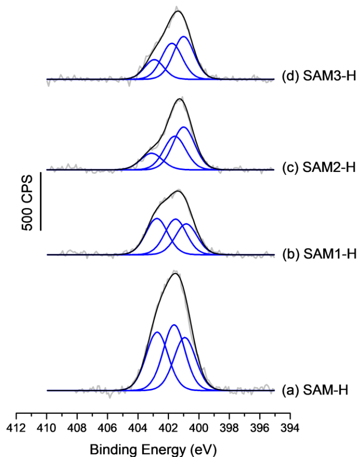
Figure 4. High resolution XPS spectra of the N1s region for triazole SAMs obtained either directly or after click reaction of SAM-N3 with heptyne: a) SAM-H (direct grafting of compound 5 ), b) SAM1-H (post-functionalized from SAM-Br), c) SAM2-H (functionalized by immersion), and d) SAM3-H (functionalized by spin coating).
