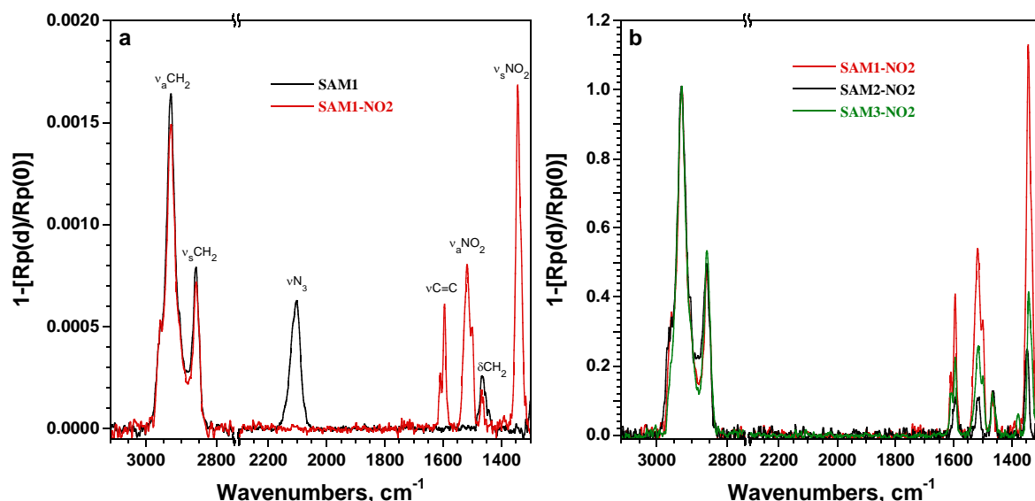
Figure 3. a) Non normalized PM-IRRAS spectra before and after the click reaction with the nitro probe for the post-functionalized SAM1 . b) Normalized PM-IRRAS spectra of SAMs after click reaction for the three methods of deposition in the 3100-1300 \text{cm}^{-1} spectral range.
