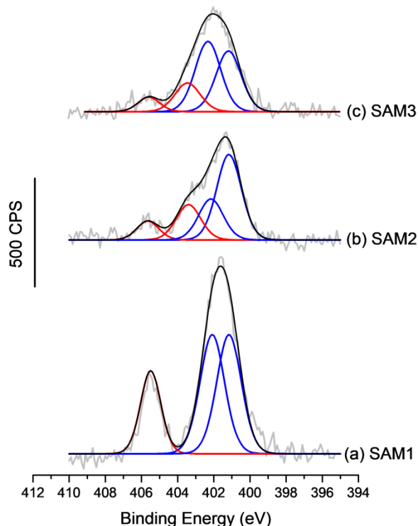
Figure 2. High resolution XPS spectra of the N1s region for SAM-N3 surfaces: a) post-functionalized SAM1 , b) functionalized by immersion SAM2 and c) functionalized by spin coating SAM3 . The blue contributions at low Binding Energy are assigned to the electron enriched ( \bar{N}=\bar{} ) and neutral ( =N- ) nitrogen atoms, while the red contribution is assigned to the electron deficient ( =N^+= ) nitrogen atoms.
