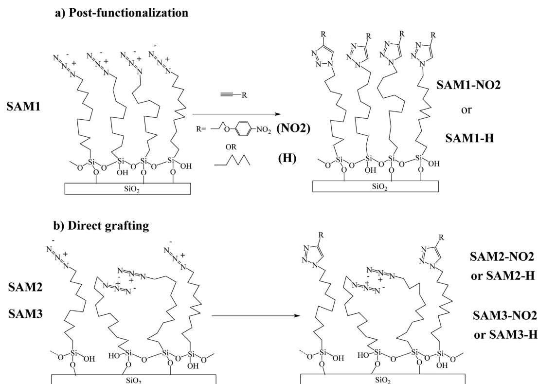
Scheme 1. Left) Schematic representation of the molecular organization inside the SAM-N3 depending of the deposition methods: a) by post-functionalization from SAM-Br (SAM1) and b) by the direct grafting of silylated coupling agent (4) by immersion (SAM2) and spin coating (SAM3) processes. Right) Schematic representation of the corresponding SAMs after click reaction with the nitro probe (SAMx-NO2) and the heptyne compound (SAMx-H).
