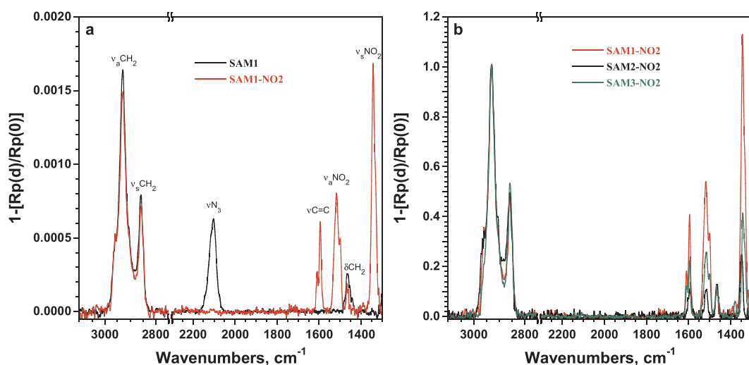
Fig. 3. a) Non normalized PM-IRRAS spectra before and after the click reaction with the nitro probe for the post-functionalized SAM1. b) Normalized PM-IRRAS spectra of SAMs after click reaction for the three methods of deposition in the 3100–1300 \text{cm}^{-1} spectral range.
