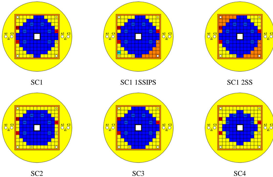
Figure 1. : Mid-plane cross-section of the VENUS-F reactor configuration studied. Fuel assemblies are in blue, Control and PEAR Rods in red, lead elements in yellow. Stainless steel is in orange. Experimental slots are in white.
