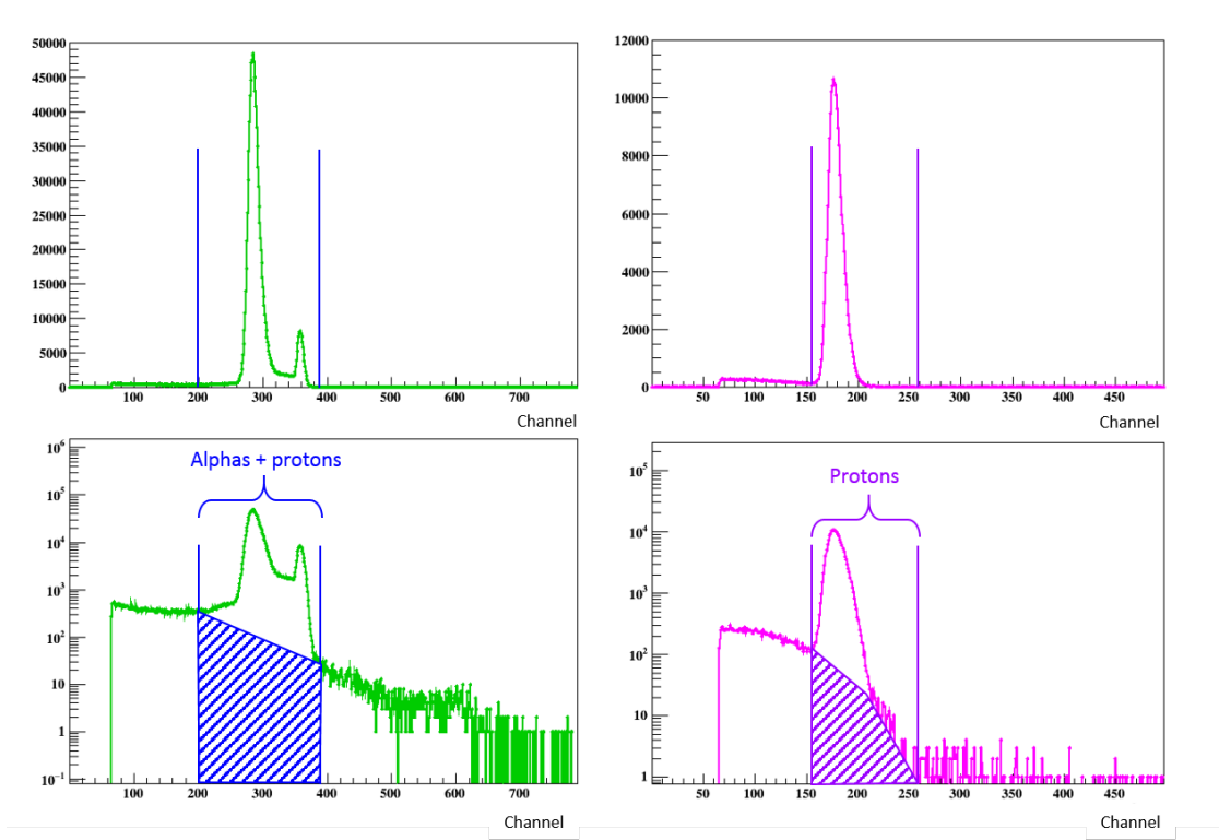
Figure 2. API and PI neutron monitor spectra in both linear and logarithmic scales. Peak area boundaries (between cursors) and subtracted background (hatched) are also shown.
