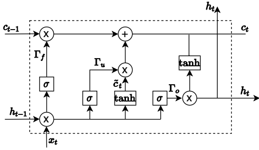
Fig. 2. Cells description of the long short-term memory implementation.
