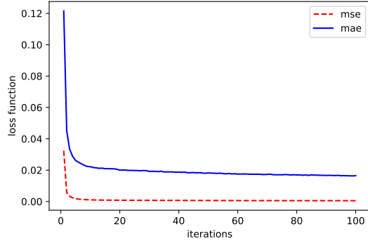
Fig. 8. Gradient of the mean square error (MSE) and the mean absolute error (MAE) as a function of the number of the number of iterations.
