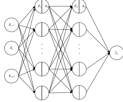
Fig. 1. Principle of the multilayer perceptron with two hidden layers.
