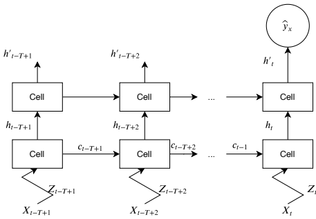
Fig. 3. Principle of the long short-term memory implementation with more than two layers.
