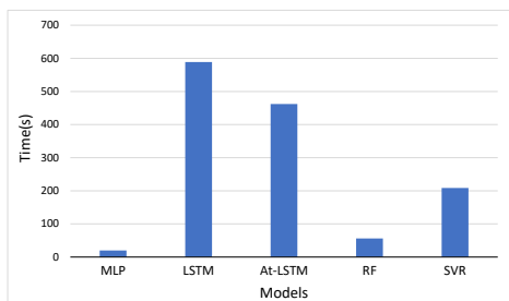
Fig. 10. Execution time of the five implemented techniques.
