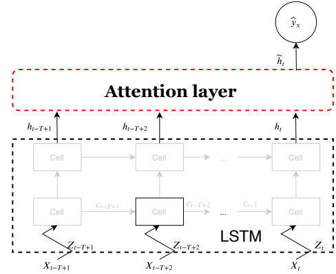
Fig. 4. Attention-based long short-term memory implementation.
