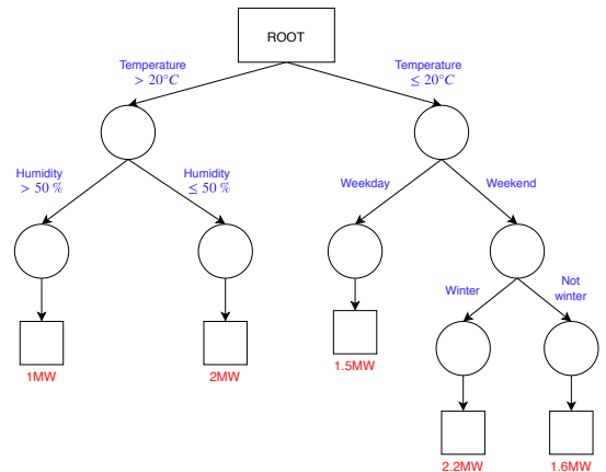
Fig. 5. Illustration of a sample random forest tree.
