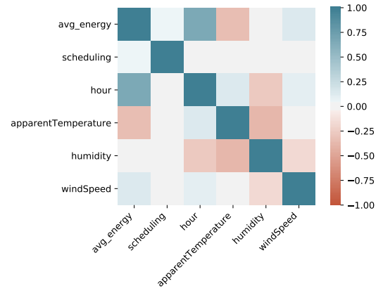
Fig. 7. Correlations of weather parameters and energy in the data-set [10].
