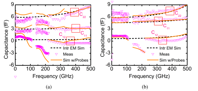
Fig. 6. All the capacitances measurement, intrinsic HFSS and complete structure simulations of the open-M1 for both Run-1 and 2. These capacitances are related to port-1 ( C_{11} ), port-2 ( C_{22} ), and the coupling capacitance between the port-1 and port-2 ( C_{12} ).
