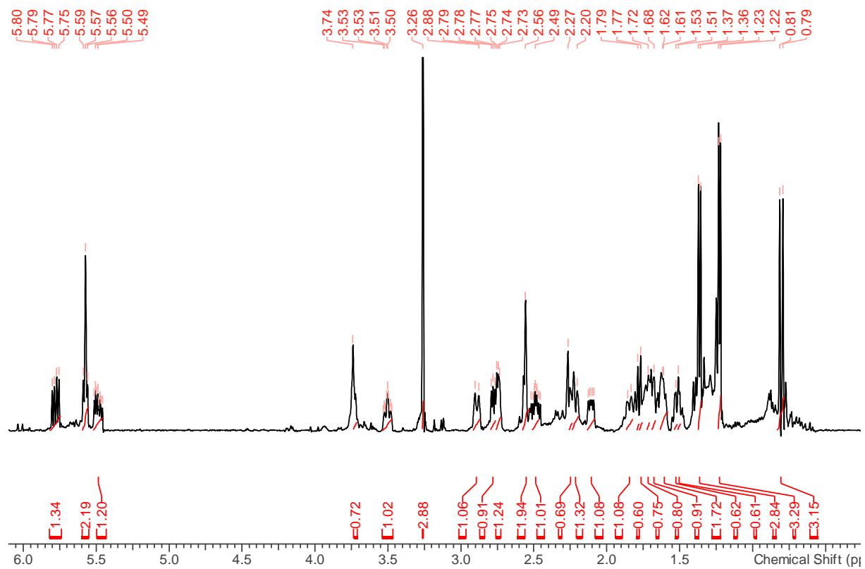
Figure S1. 1 H-NMR spectrum (500 MHz, CDCl 3 ) of compounds 1 and 2 (mixture).
