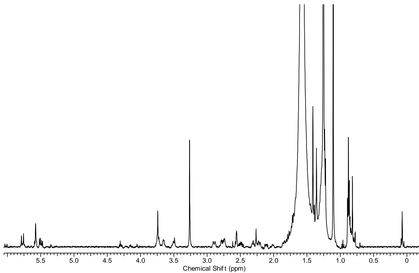
Figure S4. 1 H-NMR spectrum (500 MHz, CDCl 3 ) of compound 2.
