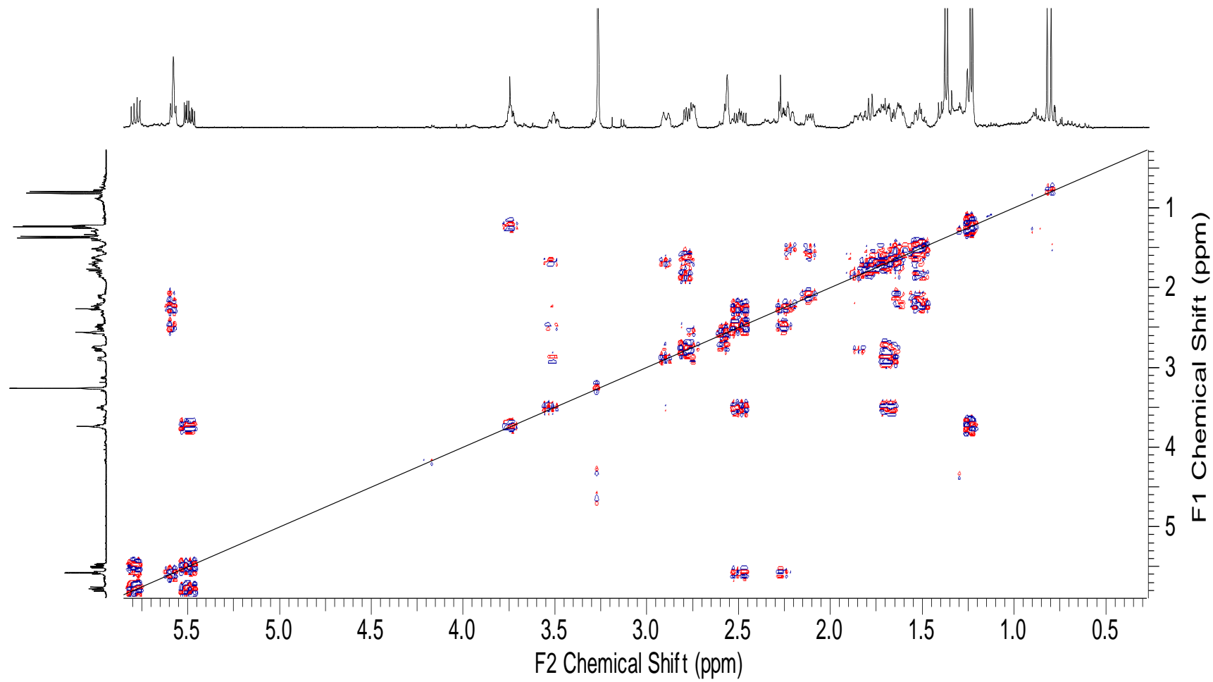
Figure S8. COSY spectrum (500 MHz, CDCl 3 ) of compounds 1 and 2 (mixture).
