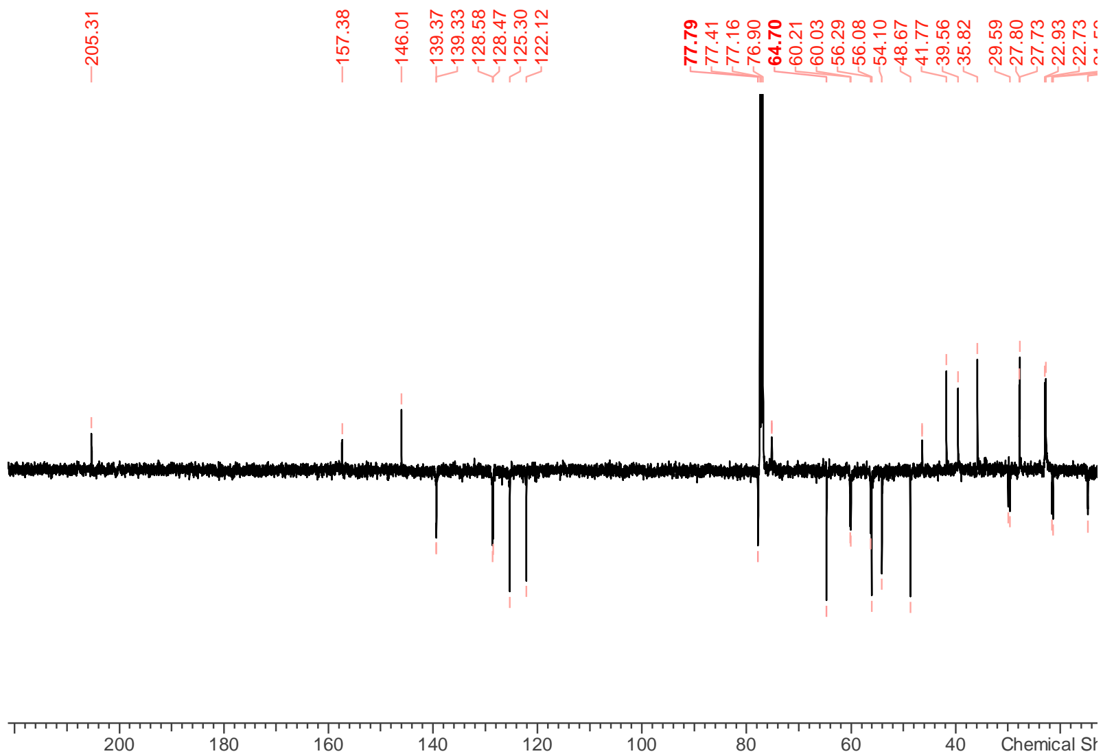
Figure S5. ^{13}\text{C} -NMR spectrum (125 MHz, \text{CDCl}_3 ) of compounds 1 and 2 (mixture).
