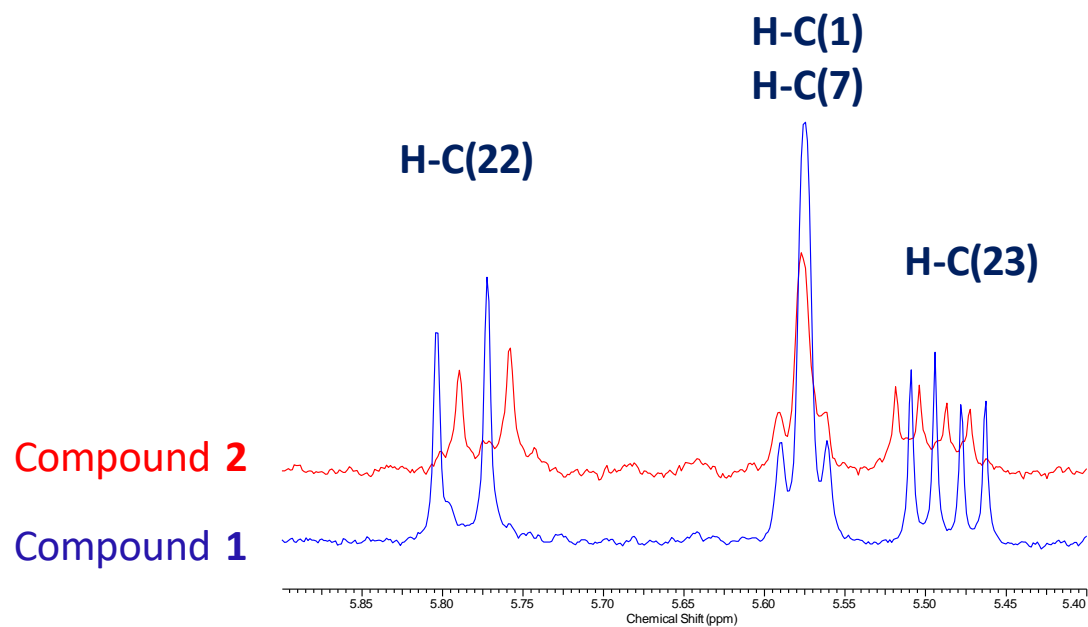
Figure S2. ^1\text{H-NMR} spectrum of the 1:1 mixture and of the HPLC-purified compounds 1 and 2 ( \delta_{\text{H}} 5.40-5.90 ppm, 500 MHz, \text{CDCl}_3 ).
