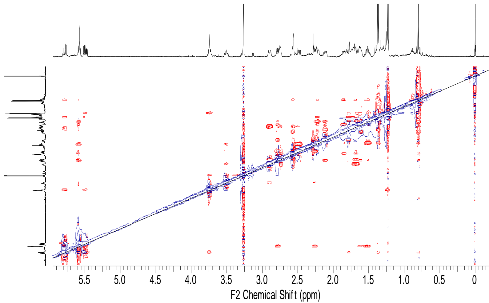
Figure S9. NOESY spectrum (500 MHz, CDCl 3 ) of compounds 1 and 2 (mixture).
