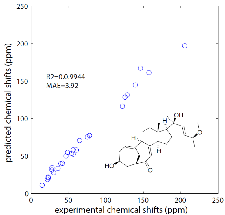
Figure S10. Comparison between experimental and DFT calculated chemical shifts for compounds 1 and 2.
