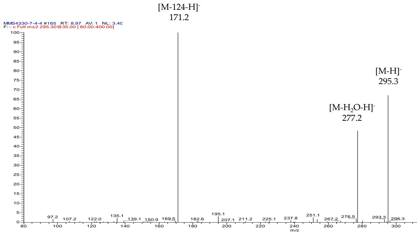
Figure S12. MS/MS spectrum of \alpha -dimorphecolic acid in negative ionization mode
