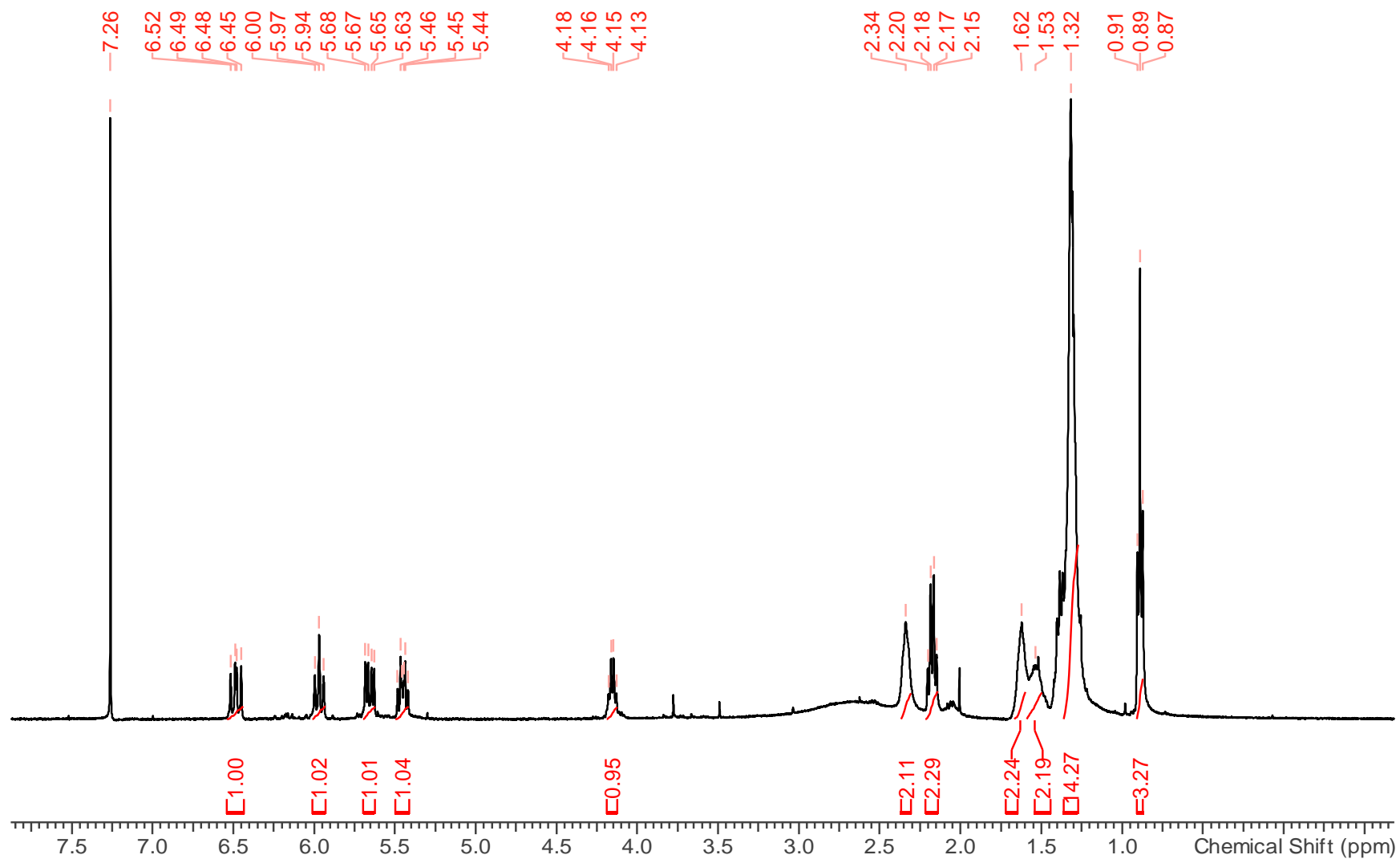
Figure S11. 1 H-NMR spectrum (500 MHz, CDCl 3 ) of α-dimorphecolic acid
