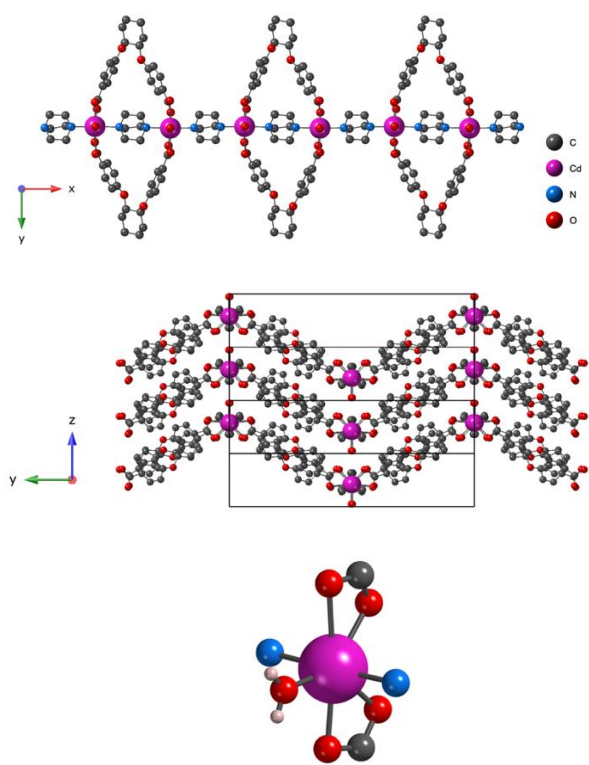
Figure 5. A portion of the chiral 1D coordination network obtained upon combining \text{Cd}(\text{NO}_3)_2 , 3b or 3c and Dabco auxiliary ligand: metallamacrocycles connected by Dabco leading to a 1D chain along the a axis (top), together with the corresponding packing (middle); coordination sphere around the metal centre (bottom).
