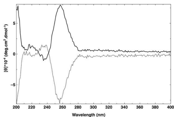
Figure 3. Circular Dichroism spectra of 3b (black solid line) and 3c (black dashed line) in CHCl 3 at RT.
