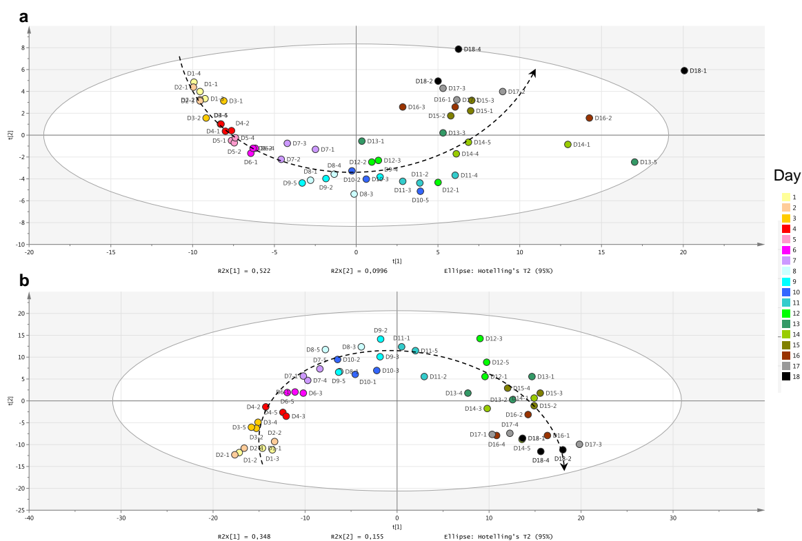
Figure 3. Principal component analysis (PCA) obtained from LC-(+)ESI-HRMS profiles corresponding to the extracts of marine-derived fungi from Day 1 (D1) to Day 18 (D18), (3 replicates per day) based on features ( m/z at R_t associated to its normalized peak area) detected in LC-MS chromatograms: (a) P. canescens MMS460; and (b) Penicillium sp. MMS388.
