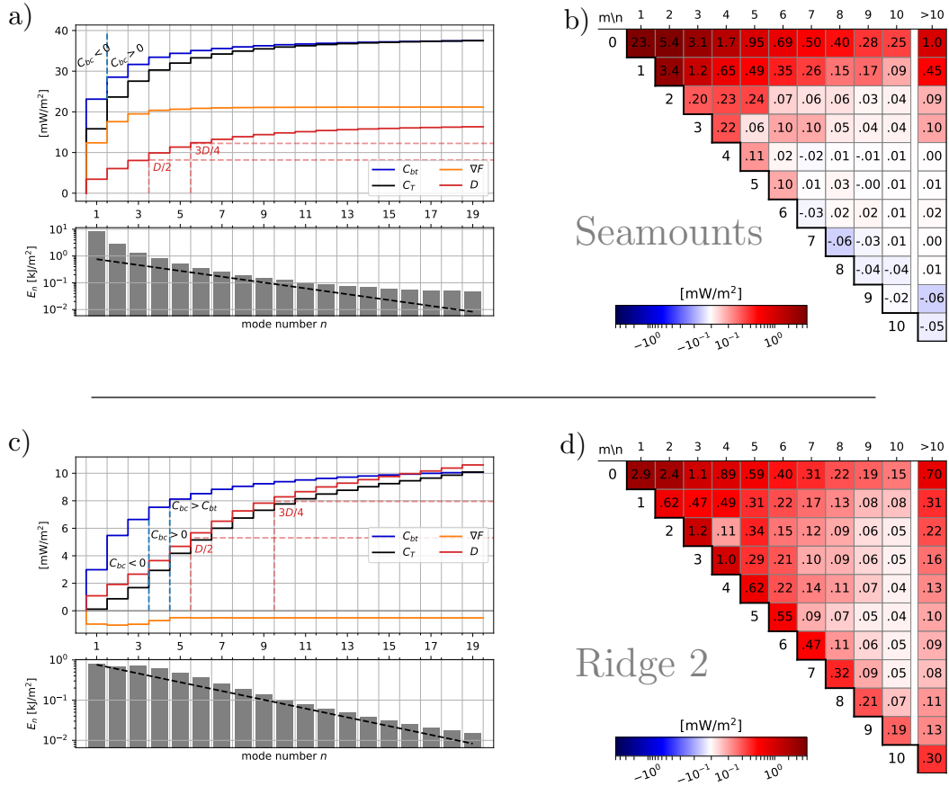
Figure 6. Same as figure 5, panels b) and c), but for "seamounts" (top: a and b) and "ridge2" (bottom: panels c and d) subdomains. Note that the extent of the vertical axis is different between panels a) and c). The black dashed curve in these panels (bottom frame) is the same as in Fig. 5 (c) for comparison.
