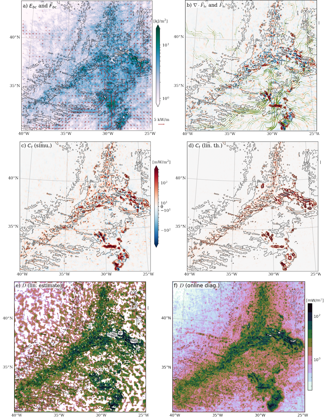
Figure 2. Energetics of the M_2 internal tide (vertically integrated): a) Baroclinic energy (colors, log scale) and energy flux (arrows). b) Divergence of the baroclinic energy flux (colors). A streamplot of the energy flux corresponding to the arrows in panel a) is superimposed. c, d) Barotropic-to-baroclinic conversion term C_t computed in the simulation and predicted by the linear solution, respectively. e) Baroclinic energy dissipation inferred from the difference between the energy flux divergence and the conversion term (model estimate, negative values appears white – see text for explanation). f) Total energy dissipation estimated from the model (online diagnostics). Plots with the same color scheme share the same colorbar.
