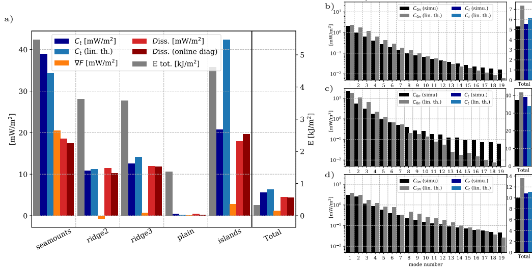
Figure 4. a) Bar plot of the different terms of the vertically-integrated baroclinic energy balance averaged in the subdomains depicted in Figure 1: Barotropic-baroclinic conversion term estimated in the model (dark blue) and from the linear solution (light blue), energy flux divergence (orange), energy dissipation estimate based on linear theory (baroclinic energy only, light red) and from online diagnostics (total energy, dark red); b-d) Barotropic modal conversion rate: model estimate and linear theory, over the entire domain (b), the seamounds domain (c) and the “ridge2” domain (d).
