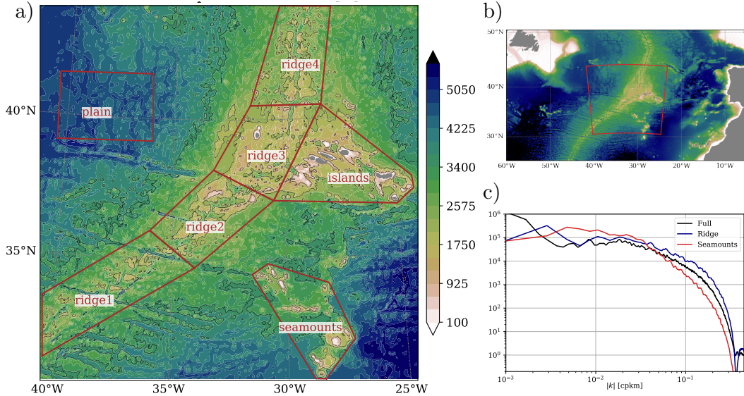
Figure 1. a) Topography used in the numerical simulations. Subdomains of particular interest are superimposed in red contours. The Azores Islands are visible in the “Islands” subdomain, and the “seamounts” subdomain corresponds to the (northern part of the) Atlantis-Great Meteor Seamount Chain; b) Bathymetry (from SRTM30-plus dataset) of a larger region of the North Atlantic, showing the location of the numerical domain; c) Spectra of the topography (variance preserving) for the entire numerical domain and in two particular regions (square domains covering the “seamounts” and “ridge2” subdomains if panel a).
