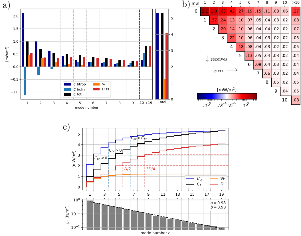
Figure 5. Internal tide scattering: a) modal energy terms averaged over the entire numerical domain, with C_{\text{bclin}} the sum of the exchanges of one mode with every other baroclinic mode, i.e. C_{\text{bclin}}^m = \sum_{m>0} C_{mn} ; b) matrix representation of the C_{mn} terms averaged in space. m (resp. n ) increases with row (resp. column) number, and the first row corresponds to the barotropic-to-mode- n conversion term. Only the upper triangle is shown, as the matrix is anti-symmetric. Energy exchanges with high modes (10 or 11 to 19) are gathered for clarity in panels a) and b). c), upper panel: cumulative modal energy terms averaged over the same domain. The difference between the dark blue and the black curve is indicative of the redistribution among modes through baroclinic scattering. Regions where baroclinic scattering is negative, positive and greater than the barotropic conversion are indicated between these two curves. Also shown are typical fractions of total dissipation and corresponding mode number for which the partial cumulative modal dissipation reaches this value. c), lower panel: mean modal energy density, with an exponential fit of the form ae^{-n/b} plotted in black dashed line.
