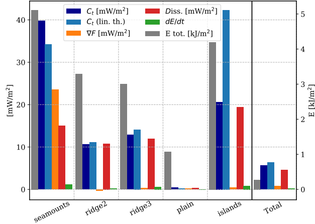
Figure 7. Vertically-integrated baroclinic energy balance per subdomain (same as Fig. 4, with online energy dissipation replaced by mean energy tendency) in the fully-realistic simulation.
