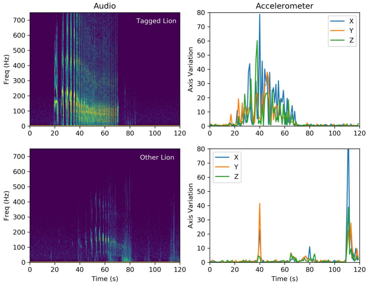
Figure 1. Concurrent audio (left) and accelerometer (right) data for two different roars recorded on the same biollogger, one emitted by the tagged lion (top row) and the other emitted by a neighbouring lion (bottom row). The combination of the audio amplitude and the clear body motion associated with roaring that is recorded by the accelerometer facilitated reliable labelling of roars according to individual identity.
