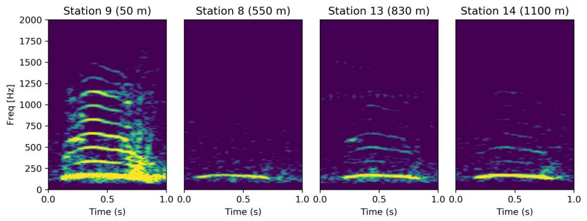
Figure 8. Spectrograms of the same FT roar recorded at varying distances from the animal.
