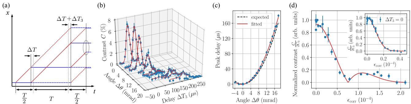
Figure 2. (a) Space-time diagram of the interferometer to introduce the definitions of the fixed \Delta T = 40 \mu\text{s} and the variable \Delta T_3 . (b) Peak-peak contrast of the spurious interferometers (blue dots) as a function of the third pulse delay \Delta T_3 , for a set of angles \Delta\theta , and Gaussian fits (solid red lines) to the corresponding data. (c) Fitted values of \Delta T_3 yielding maximum contrast for the probed values of \Delta\theta . Dashed black line is the expectation of \Delta T_3 = 2\epsilon(T + t_1) , solid red line is the fit to the data accounting for initial angular offsets \Delta\theta_{0z} , \Delta\theta_{0y} . (d) Normalized fitted peak contrast for the probed values of \epsilon_{\text{corr}} = \frac{1}{2}((\Delta\theta - \Delta\theta_{0z})^2 - \Delta\theta_{0y}^2) . The solid red line is the fit with Eq. 5 with \sigma_r and C_0 as free parameters (see text). Inset: contrast decay for \Delta T_3 = 0 . The solid red line is the expectation for the measured value of \sigma_v and the fitted value of \sigma_r .
