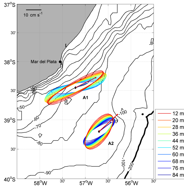
Figure 3. Bathymetry (m; GEBCO, corrected by measurements from SHN) in the mooring area; A1 and A2 sites are indicated by the black diamonds. Thin black lines represent isobaths every 10 m from 10- to 100-m depth. The 200-m isobath is indicated by the heavy black line. Also shown are the variance ellipses of in situ currents at all sampled depth levels (reference scale at right). The record-length mean of the shallowest and deepest velocity at each site are indicated by arrows (reference scale on top left corner).
