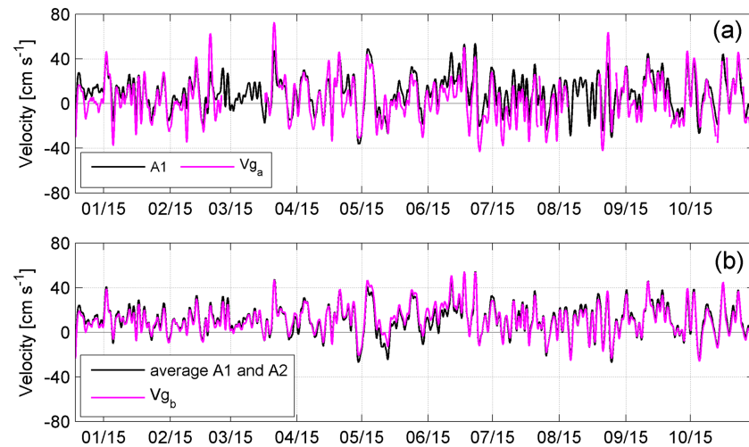
Figure 11. (a) Along-shore barotropic component at A1 excluding the Ekman layer (black) and absolute geostrophic velocity computed from SSH gradients between TG and A1 (magenta). (b) Along-shore barotropic component of the velocity excluding the Ekman layer (black) averaged over A1 and A2 and absolute geostrophic velocity computed from SSH gradients between A1 and A2 (magenta).
