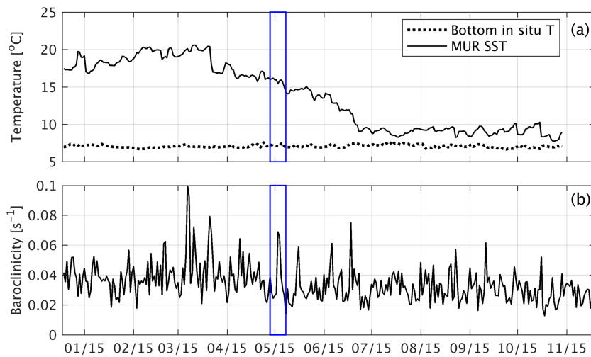
Figure 9. Same as Figure 8 at A2.
