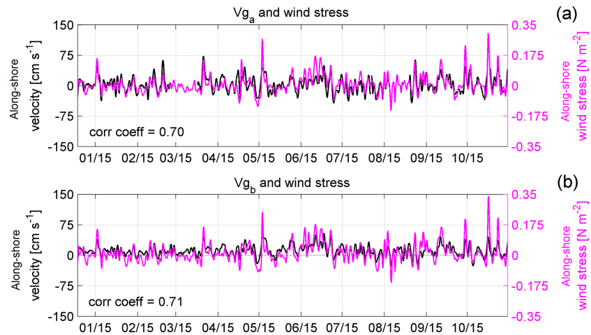
Figure 12. Along-shore absolute geostrophic velocity (black line) (a) between TG and A1 and (b) between A1 and A2, alongshore and wind stress from ERA-Interim (magenta line). See Figure 1 for reference.
