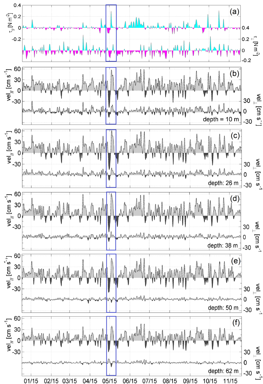
Figure 4. (a, top) Along- and (bottom) cross-bathymetry wind stress ( \text{N/m}^2 ) at A1 from ERA-Interim. (b–f) Along- and cross-bathymetry velocity ( \text{cm/s} ) at selected depths at A1. The blue rectangle indicates the timing of an extreme flow reversal event described in section 4.3. Along-bathymetry velocities are positive toward the ENE and cross-bathymetry velocities are positive toward the WNW (onshore).
