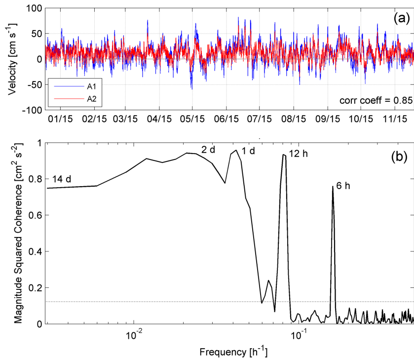
Figure 6. (a) Nonfiltered alongshore barotropic velocity time series at A1 (blue) and A2 (red) and (b) coherence spectrum. The horizontal dashed line in (b) represents the 95% confidence level.
