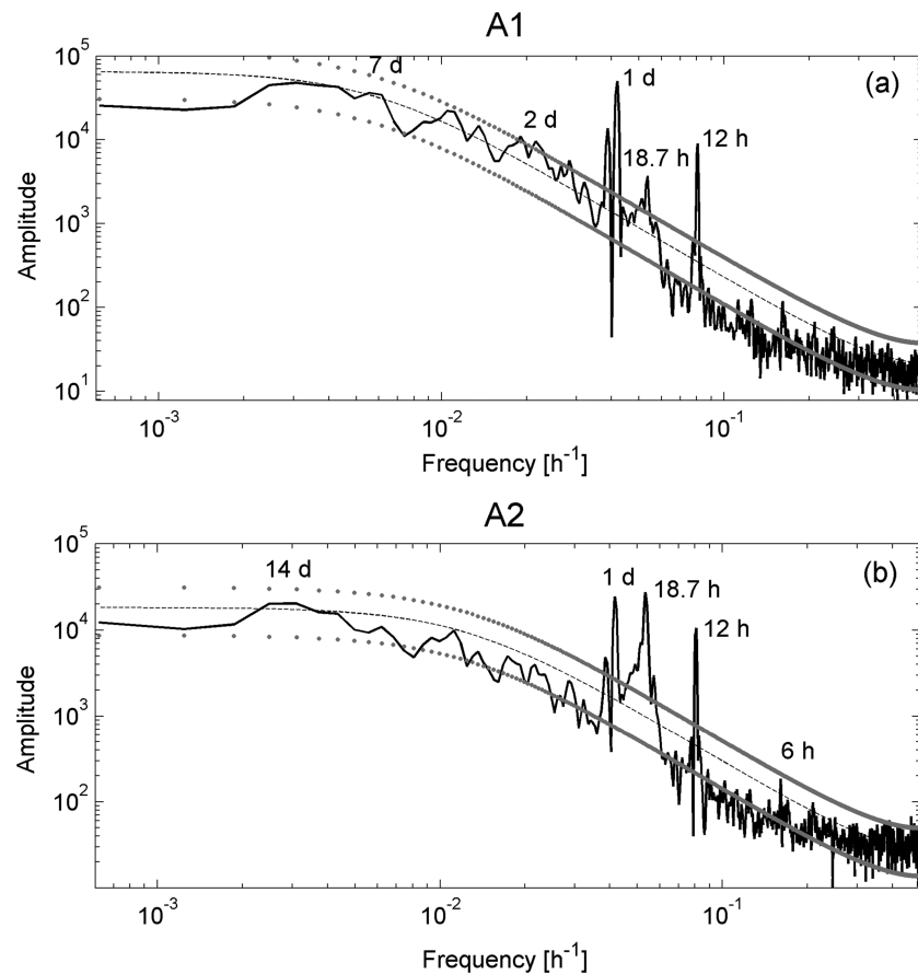
Figure 2. Along-bathymetry current spectra from the shallowest level, (a) 10 m at A1 and (b) 12 m at A2. The dotted lines indicate the 95% confidence level.
