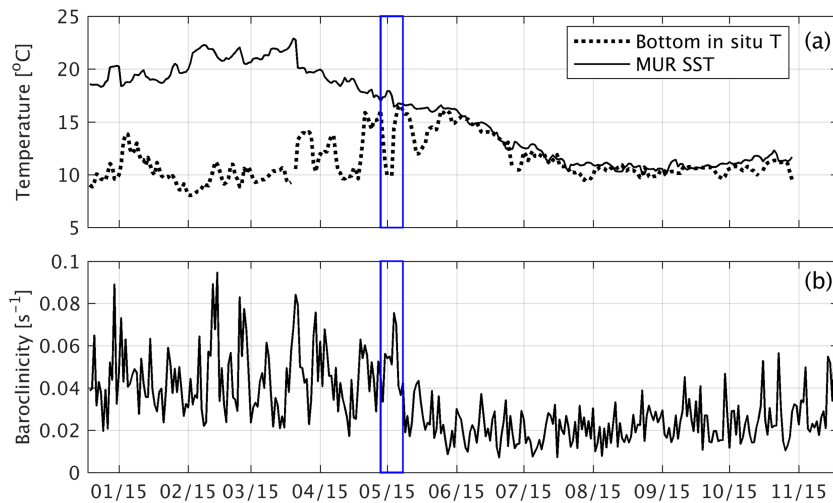
Figure 8. (a) Satellite SST (thin line) and in situ bottom T (dashed line) at A1. (b) Baroclinicity index from in situ velocities. The blue rectangle indicates an extreme flow reversal event described in section 4.5.
