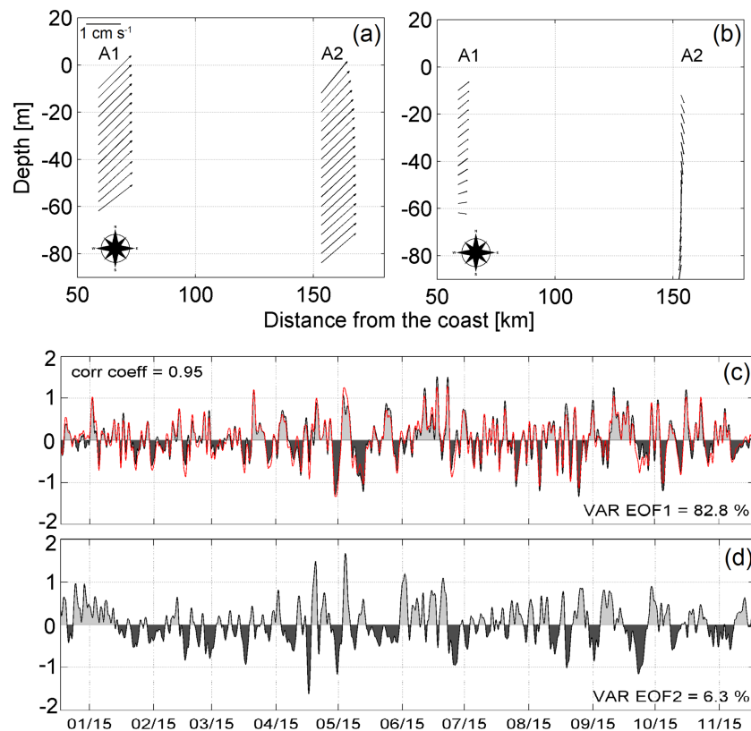
Figure 7. Spatial patterns and normalized time series of the (a and c) first and (b and d) second EOF mode of the barotropic velocity component at A1 and A2. The red line in (c) shows the normalized alongshore barotropic velocity at A1. Vectors shown in (a) and (b) represent the geographical direction in the horizontal plane (zonal and meridional), and the axis indicates the location associated with each vector (to what deployment and what depth level each horizontal vector corresponds).
