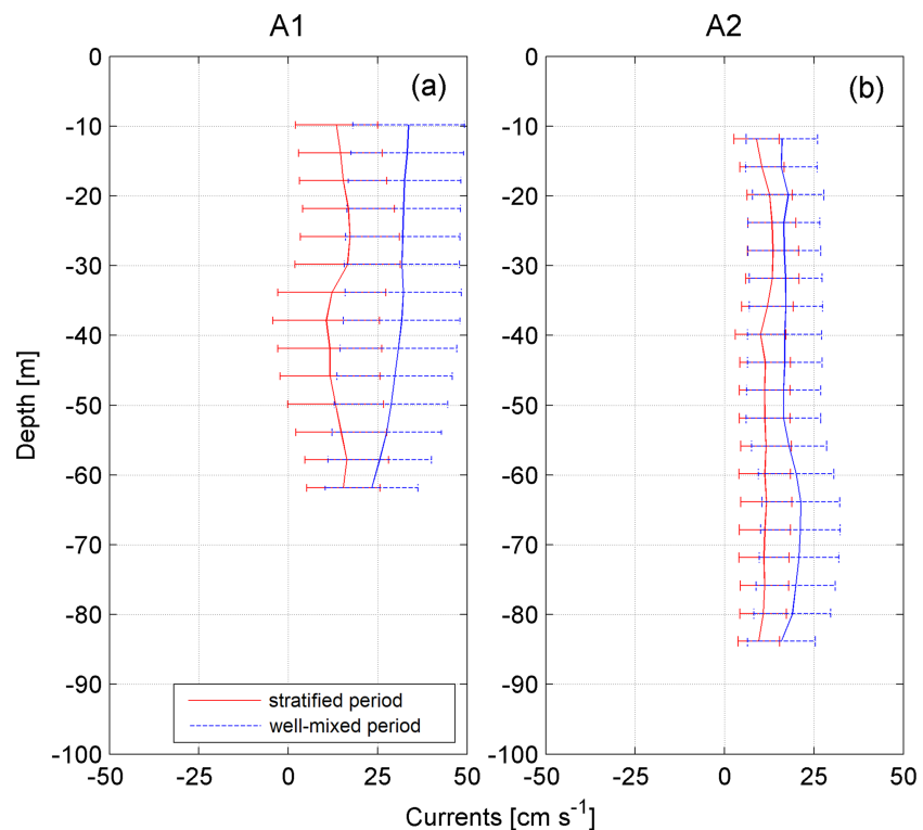
Figure 10. Time-averaged velocity and standard deviation of the alongshore currents for the stratified period (red) and the well-mixed period (blue) at (a) A1 and (b) A2.
