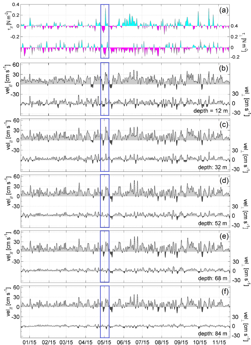
Figure 5. Same as Figure 4 at A2.
