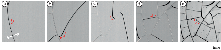
Figure 4: Hierarchical crack formation. Invasion of the plane of the layer by successive generations of cracks. From left to right: first, second, third and fourth order. In each image of the sequence a-d , the cracks of higher orders are highlighted in black; in each image the red arrows highlight one particular crack of a new generation. The final pattern is shown in (e).
