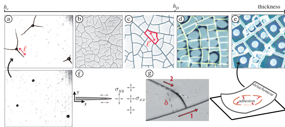
Figure 3: Crack networks as a function of the layer thickness (each image exhibit final crack patterns). (a) Star-like patterns with 3 branched cracks at 120^\circ each other nucleated from nucleation sites (bubbles in the bottom image). (b) Broken network of cracks. (c) Close network of cracks limiting domains. (d,e) Partial delamination from the substrate confined at the edge of the domains (d); for thicker layers, inside a particular domain the circular optical interference fringes display an air gap and encircle an adhering region (bright area in (e)). (f) Sketch of the growth of cracks in an initially homogeneous stretched medium. (g) When a crack (2) propagates in the vicinity of a pre-existing crack (1), the crack path (2) is modified to take into account the stress release of (1).
