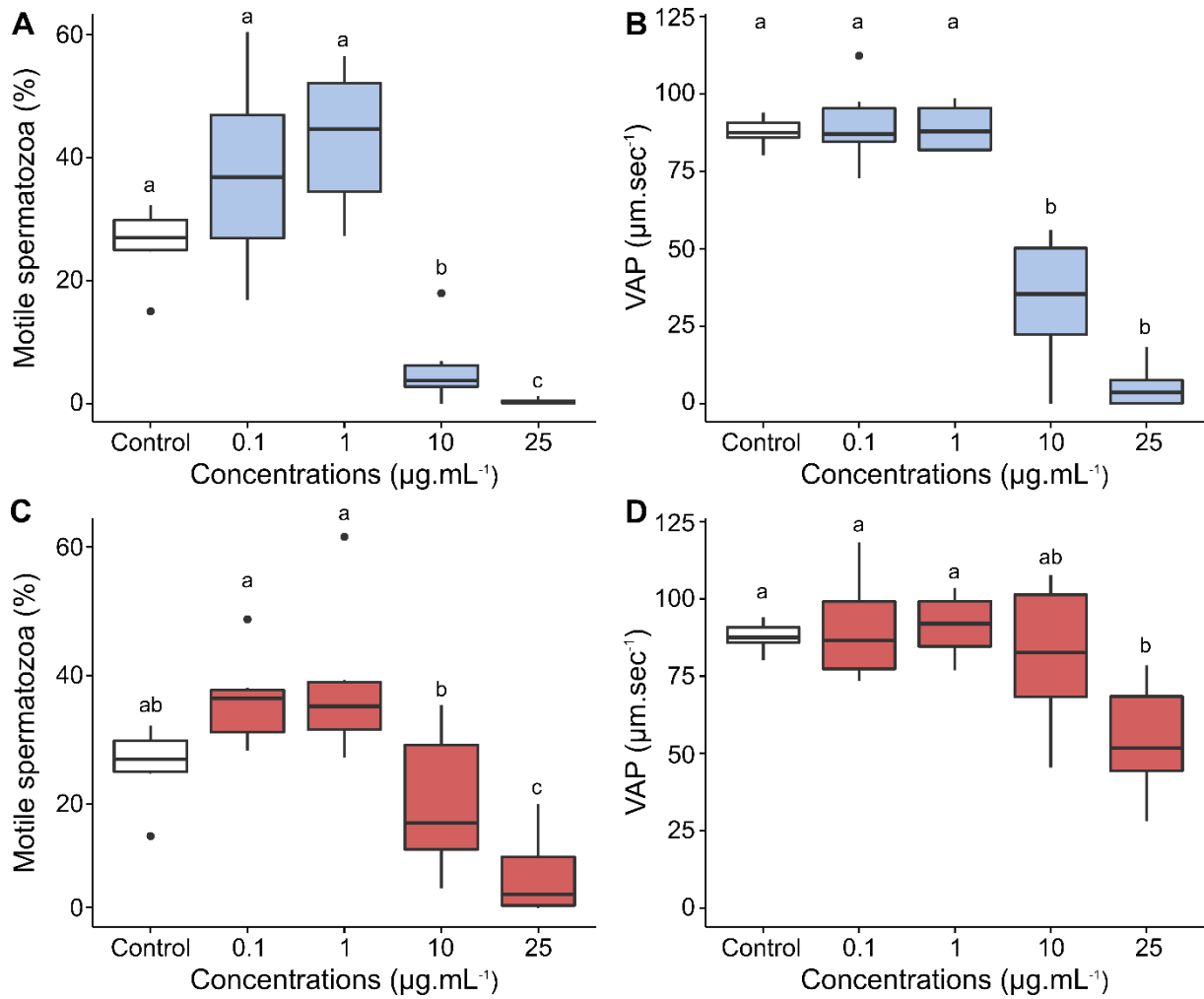
Figure 2. Percentage of motile spermatozoa (%; A and C) and velocity of the average path (VAP; \mu\text{m}\cdot\text{sec}^{-1} ; B and D) of oyster spermatozoa after 1 h of exposure to 50-NH 2 (blue, A and B) and 50-COOH beads (red, C and D) at five concentrations: 0 (Control), 0.1, 1, 10, and 25 \mu\text{g}\cdot\text{mL}^{-1} . N = 6. ANOVA (A, C and D) or Kruskal-Wallis tests (B) with pairwise comparisons were made between treatments at the 5% level; homogeneous groups share the same letter.
