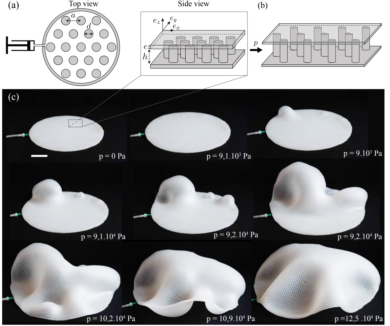
FIG. 1: Elastic phase separation. (a) (left) Schematic top view of the regular pillar lattice of pitch a , the diameter of the pillars being d . The boundary walls have a thickness of approx. a/2 . The structure is connected to a pressure supply (e.g. a syringe). (right) Schematic 3D representation of a portion of the structure, e being the thickness of the top and bottom membranes, and h the height of the pillars. (b) Upon inflation, the structure deforms, changing thus the actual \psi and \phi parameters, leading to geometric non-linearities. In the model proposed, the deformed pillars are approximated by cylinders, neglecting the boundary effect on the actual shape of the pillar, and accepting the deformation mismatch at the boundary pillar-membrane (the pillars shrink in the xy -plane, whereas the membrane is stretched). (c) Series of pictures of a large plate embedding a regular hexagonal lattice of pillars upon inflation (diameter of 25 cm, a=3 mm, d=2.4 mm, h=3 mm, e=1.2 mm). Bulges appear in the plate and then propagate through the whole structure, at a nearly constant pressure. Scale bar: 5 cm.
