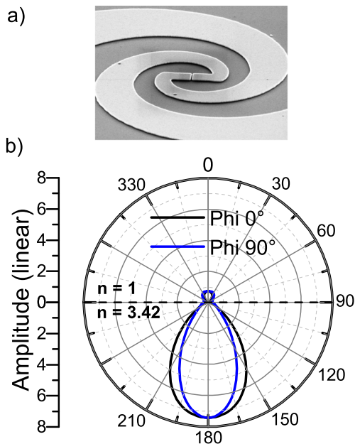
FIG. 3. (a) SEM picture of the double-helix log spiral antenna of the HEB. (b) Numerical simulation of the beam pattern of our log-spiral antenna at the interface of two infinite dielectric half spaces with index of refraction n_{\text{air}} = 1 for the upper half space and n_{\text{HR-Si}} = 3.4 (HR-Si at 2.7 THz) for the lower half space, respectively.
