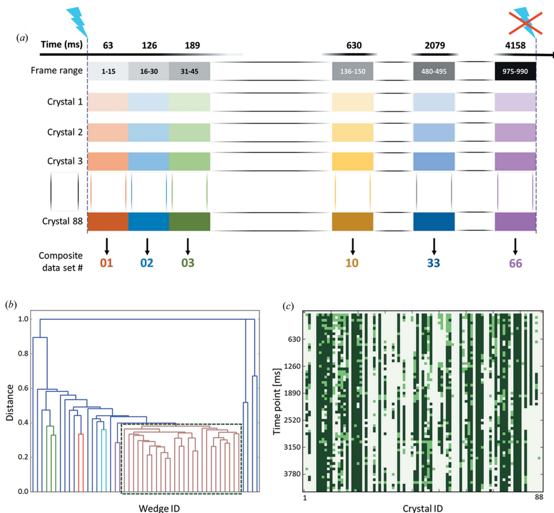
Figure 2 Data-collection strategy and data set composition. (a) Complete data sets were collected from 88 different crystals. For each crystal, the diffraction images were separated into 15 frame wedges corresponding to 66 time points (from 63 to 4158 ms). (b) A dendrogram of wedge clustering for the initial time point ( t = 0\text{--}63 ms). The 26 wedges forming the cluster highlighted with a dark green rectangle group at a linkage distance of 0.39 were subsequently merged together to produce a 2.45 Å resolution data set with 100% completeness and a multiplicity of 12.6 (Table S1). (c) A visualization of the data set wedges integrated (light and dark green) and of the wedges retained in the composite data sets corresponding to the 66 different time points (dark green only).
