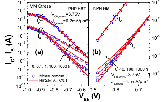
Fig. 5: Comparison between measurement and HiCuM-AL-V3.1 simulation: Gummel plots at different aging intervals for (a) PNP HBTs under J_{E, stress} of 6.2 \text{ mA}/\mu\text{m}^2 and V_{CB, stress} of 3.75 \text{ V} and (b) NPN HBTs under J_{E, stress} of 4.5 \text{ mA}/\mu\text{m}^2 and V_{CB, stress} of 3.75 \text{ V} .
