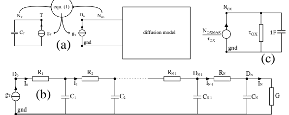
Fig. 2: Organization of the (a) R-D, (b) Diffusion model [11] and (c) Oxide-trapping model implementations.
