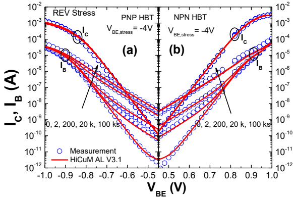
Fig. 7: Comparison between measurement and HiCuM-AL-V3.1 simulation: Gummel plots at different aging intervals for (a) PNP HBTs and (b) NPN HBTs under V_{EB, stress} of 4V.
