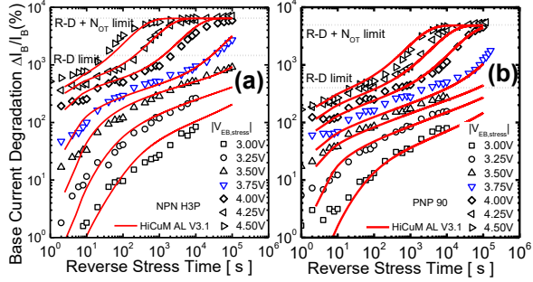
Fig. 6: Comparison between measurement and HiCuM-AL-V3.1 simulation: Evolution of excess base current extracted at V_{BE} = 0.7 V for (a) NPN HBTs and (b) PNP HBTs under different V_{EB, stress} (3 - 4.5V).
