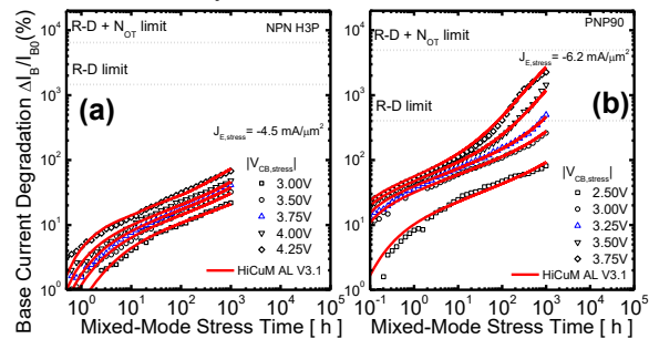
Fig. 4: Comparison between measurement and HiCuM-AL-V3.1 simulation: Evolution of excess base current at V_{BE} = 0.7 V for (a)
