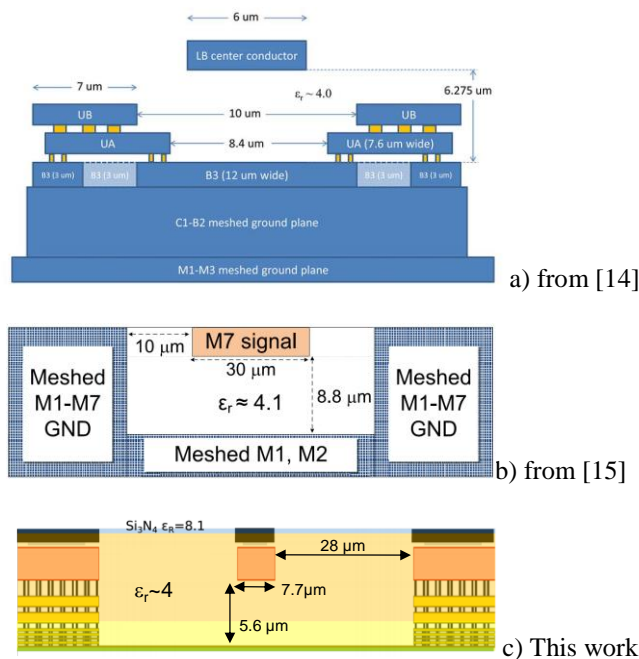
Fig. 2. Cross-sectional view of different lines used in on-wafer calibration kit: a) line fabricated in 45nm CMOS SOI process[14], b) CPWG line fabricated in a IHP Bipolar process[15], c) microstrip line fabricated in BiCMOS 55nm STMicroelectronics process. (copyright to be done)
