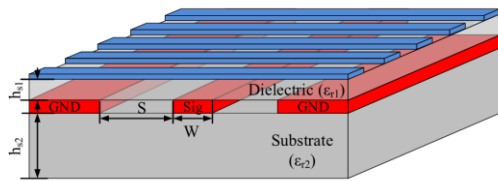
Fig. 5. Simplified sketch of a CL-ICPW section. The transmission line consists of a CPW realized on the lossy substrate, which is characterized by a dielectric constant \epsilon_2 and is capacitively loaded by means of floating bars separated by a dielectric layer, with dielectric constant \epsilon_1 . Extracted from [7] (copyright to be done)
