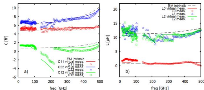
Fig. 13. (a) Capacitances of the transistor-open; (b) Inductors of the transistor-short. In both the panel, measurement (symbols), virtual measurement (EM with probe and calibration represented by solid line) and EM intrinsic simulation (dashed line) are shown up to 500 GHz
