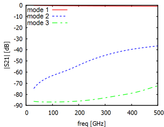
Fig. 3. Simulation of the first 3 modes of the micro-strip line from Fig. 2c (without pad) highlighting that only the first mode is propagated within the line (Length= 583\mu\text{m} ).
