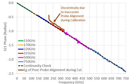
Fig. 14. Phase versus frequency ( -0.185 \text{ Deg/GHz} ) for the 0.5ps Line extracted from [32].
