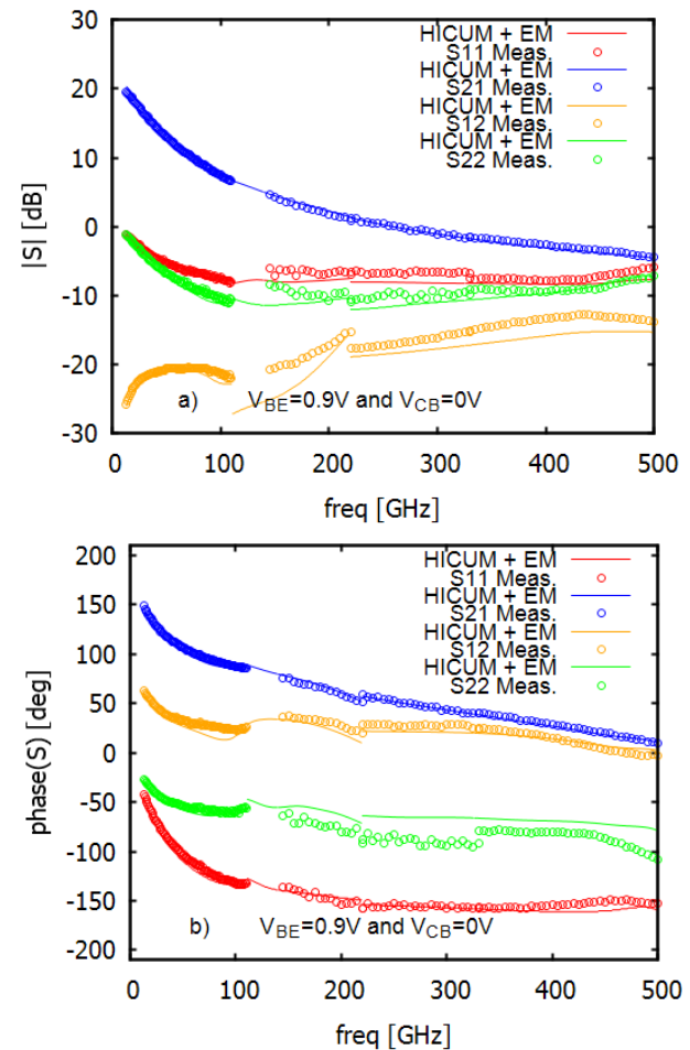
Fig. 17. Magnitude and phase of the S-parameters of a SiGe HBT for V_{\text{BE}}=0.9 \text{ V} V_{\text{CB}}=0 \text{ V} . In the figures, measurement result is shown by symbols, EM-HICUM with probe with calibration-de-embedding are shown by solid lines. Both actual measurement and virtual measurement data are calibrated using an on-wafer calibration followed by a de-embedding technique where structures are fabricated using B55 technology- STMicroelectronics.
