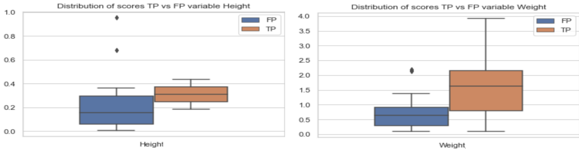
Figure 4: Comparison of (un-normalized) Scores J(eMB) distribution for variables Height and Weight for real (TP) and false detections
