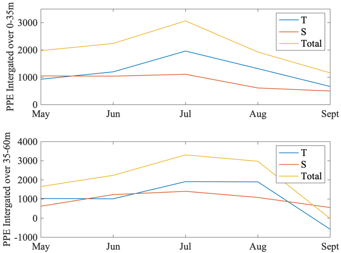
460 Figure 8: Integrated perturbation potential energy on the top 35m of the water column (a) and on the 35-60m (b). 461 PPE is represented in yellow; orange and blue describe respectively the contribution of salinity and temperature.
