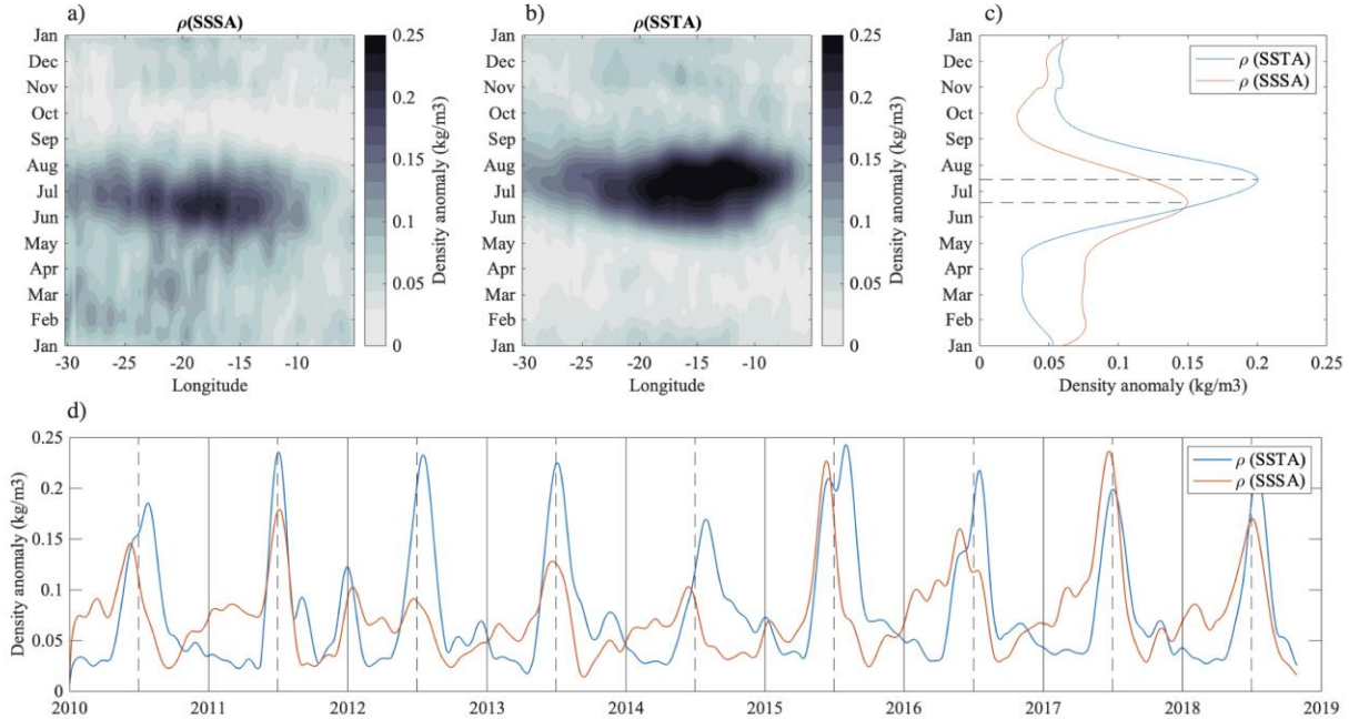
361 Figure 5: Hovmöller diagrams of the 2010-2018 climatological SSSA (a) and SSTA (b) amplitudes contributions to 362 surface density at 1^\circ\text{N} . (c) corresponding 30^\circ\text{W} - 5^\circ\text{W} longitude averaged climatologies for the contribution of SSS 363 (orange) and SST (blue). (d) 9-year time series of the contribution of SSSA (orange) and SSTA (blue) to density 364 averaged over 30^\circ\text{W} - 5^\circ\text{W} longitude.
