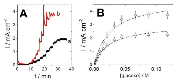
Figure 5. (A) Chronoamperometric measurements performed at E_p = 0.2 V for (a) pyreneNHS-based BP and (b) polynorbornene-based BP with immobilized thionine and FAD-GDH after addition of successive amounts of glucose with stirring in 0.1 mol L -1 PB pH 7, 25 °C; (B) Evolution of the current density with the glucose concentration accompanied with a fitting curve using a classic Michaelis-Mentens dependence. Error bars correspond to one standard deviation from at least two electrodes.
