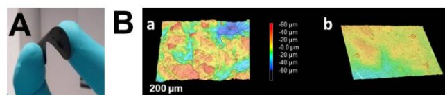
Figure 2. (A) Photograph of the flexible free-standing polynorbornene/MWCNT BP; (B) laser scanning microscopy image of the surface topography of (a) pyreneNHS BP and (b) polynorbornene BP
