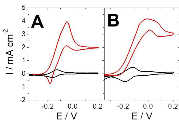
Figure 4. CV scans recorded before and after addition of 150 mmol L -1 glucose for (A) pyreneNHS-based BP and (B) polynorbornene-based BP with immobilized thionine and FAD-GDH (1 mV s -1 , 0.1 mol L -1 PB, pH 7, 25°C).
