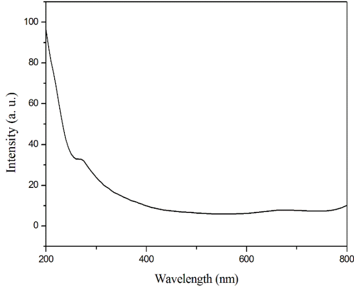
Fig. 11. Diffusion reflectance spectrum of dichlorotris(2-aminomethylpyridine)nickel(II) dihydrate at room temperature.
