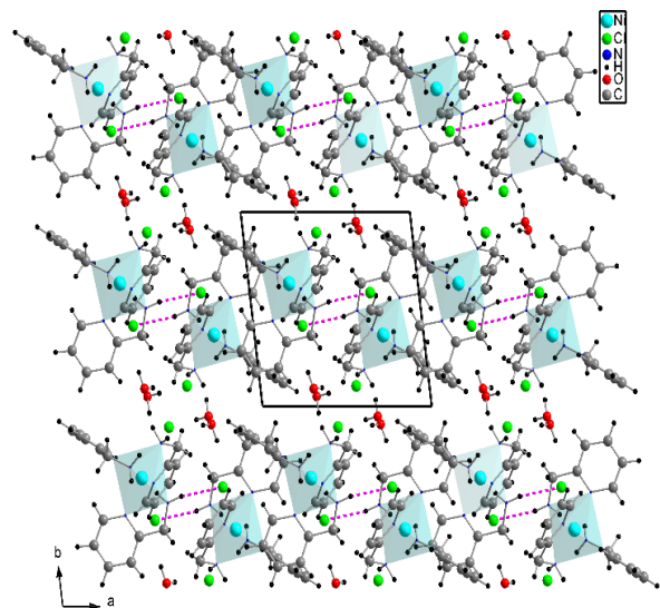
Fig. 2. N-H...Cl interactions in the (001) plane in the structure of [\text{Ni}(\text{C}_6\text{H}_8\text{N}_2)_3]\text{Cl}_2 \cdot 2\text{H}_2\text{O} .
