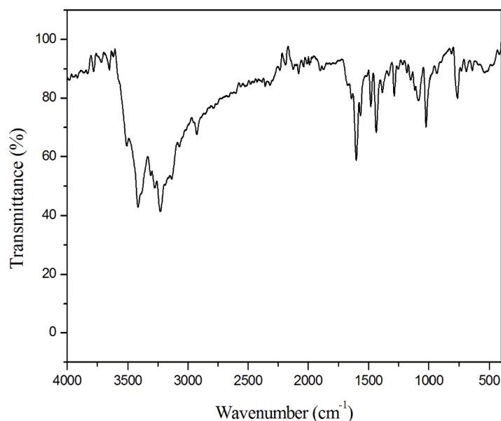
Fig. 10. Infrared spectrum of the [\text{Ni}(\text{C}_6\text{H}_8\text{N}_2)_3]\text{Cl}_2 \cdot 2(\text{H}_2\text{O}) complex.
