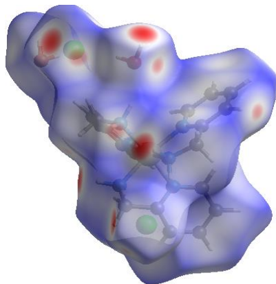
Fig. 7. 3D Hirshfeld surface mapped over d_{\text{norm}} for visualizing the molecular interactions of the studied complex. The surface is shown as transparent to allow visualization of the orientation and conformation of the functional groups.
