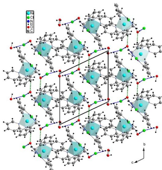
Fig. 3. O-H...Cl; N-H...O interactions in the (100) plane in the structure of [\text{Ni}(\text{C}_6\text{H}_8\text{N}_2)_3]\text{Cl}_2 \cdot 2\text{H}_2\text{O} .
