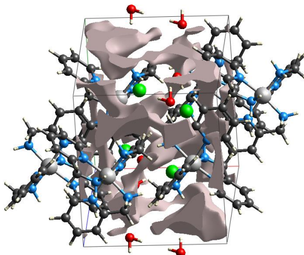
Fig. 9. The voids in the crystal structure of dichlorotrakis(2-aminomethylpyridine)nickel(II) dihydrate.
