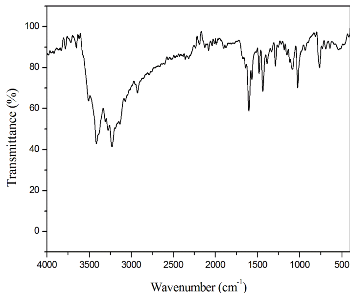
Fig. 10. Infrared spectrum of the [\text{Ni}(\text{C}_6\text{H}_8\text{N}_2)_3]\text{Cl}_2 \cdot 2(\text{H}_2\text{O}) complex.
