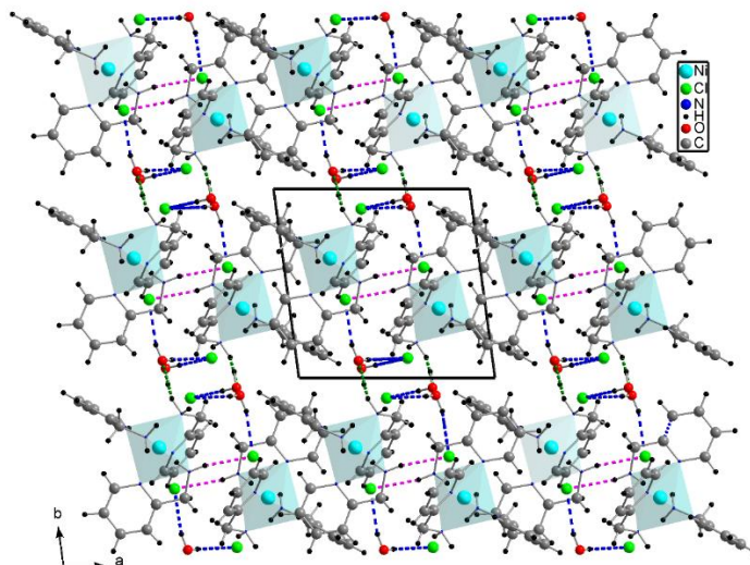
Fig. 4. 3D hydrogen-bonded supramolecular network formed by hydrogen bonding interactions (Hydrogen bonds are represented by dashed lines).
