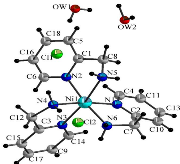
Fig. 1. The asymmetric unit of [\text{Ni}(\text{C}_6\text{H}_8\text{N}_2)_3]\text{Cl}_2 \cdot 2\text{H}_2\text{O} .
