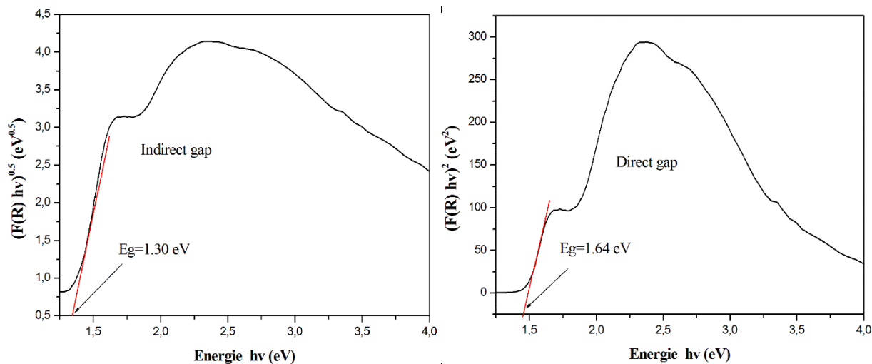
Fig. 12. Tauc Plots of (F(R) hv)^{1/2} versus E (a) and (F(R) hv)^2 versus E (b) of dichlorotris(2-aminomethylpyridine)nickel(II) dihydrate.
