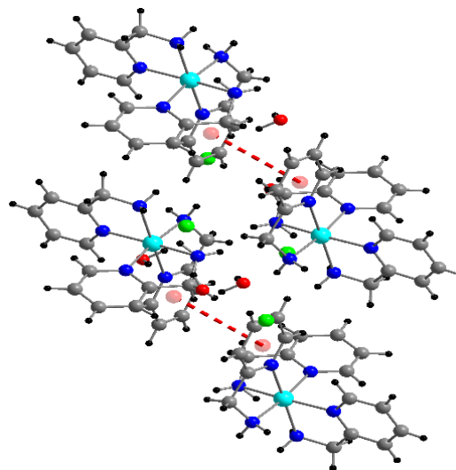
Fig. 5. The cycle stacking interaction.
