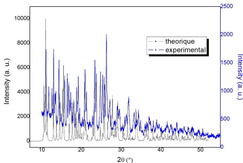
Fig. 6. Experimental and calculated diffractograms of [\text{Ni}(\text{C}_6\text{H}_8\text{N}_2)_3]\text{Cl}_2 \cdot 2\text{H}_2\text{O} .
