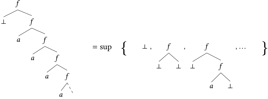
Fig. 5. The value tree of the recursion scheme \mathcal{S}
