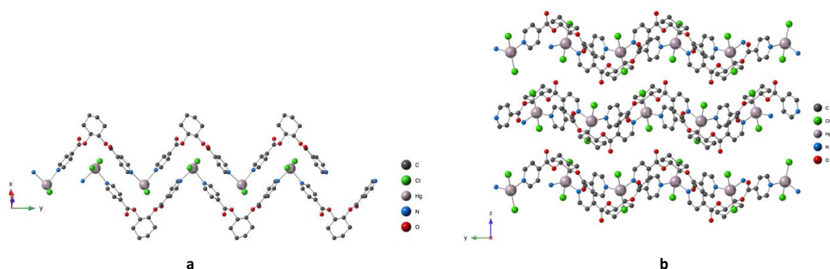
Figure 5. A portion of the chiral 1D coordination network 1a 0.5 1b 0.5 -HgCl 2 (a) and corresponding packing (b) obtained upon combining HgCl 2 with 1a+1b in racemic conditions. H atoms are omitted for clarity of the representation.
