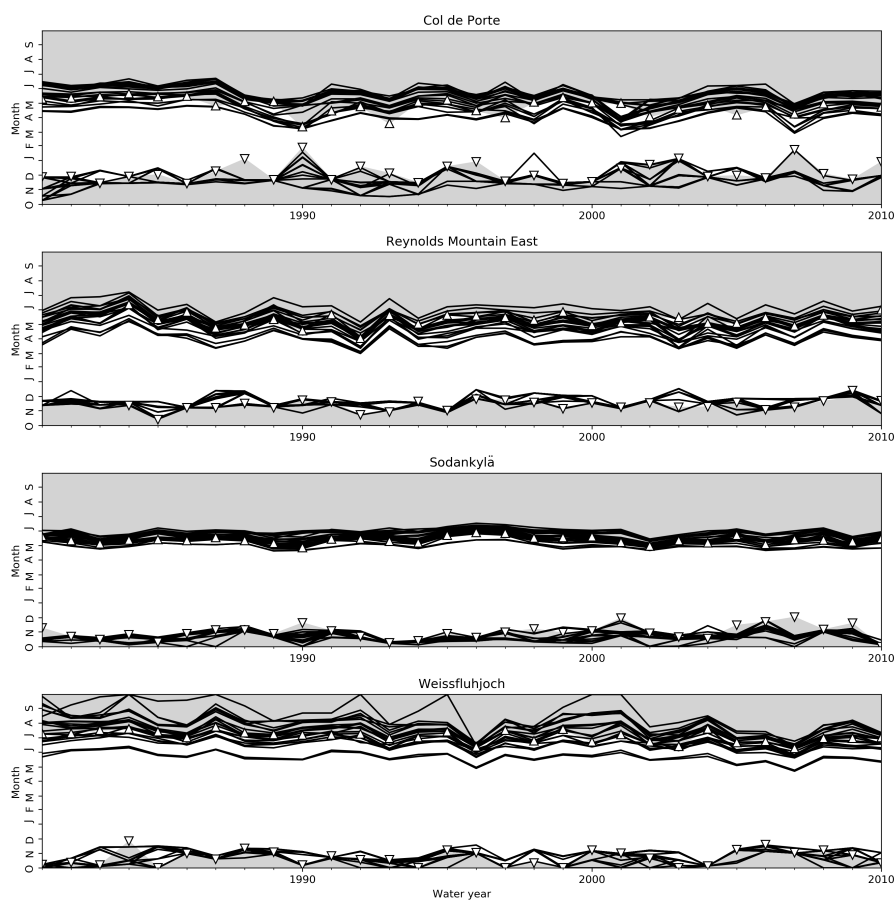
Figure A1. ESM-SnowMIP model predictions (lines) compared with observed start ( \nabla ) and end ( \triangle ) dates of continuous seasonal snow cover at the sites. Snow-free periods are shaded (ephemeral summer snow cover is not shown).
