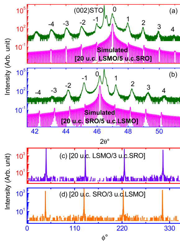
FIG. 1. \theta-2\theta x-ray diffraction pattern of (a) [\text{20 u.c. LSMO/5 u.c. SRO}]_{\times 15} and (b) [\text{20 u.c. SRO/5 u.c. LSMO}]_{\times 15} superlattices. The (002) Bragg's reflection of STO, as well as the satellite peaks (0th and \pm 4 th orders), is indicated. The diffraction profile of these superlattices calculated using the DIFFaX program is also shown. \phi scan of the (103) of the (c) [\text{20 u.c. LSMO/3 u.c. SRO}]_{\times 15} and (d) [\text{20 u.c. SRO/3 u.c. LSMO}]_{\times 15} superlattices.
