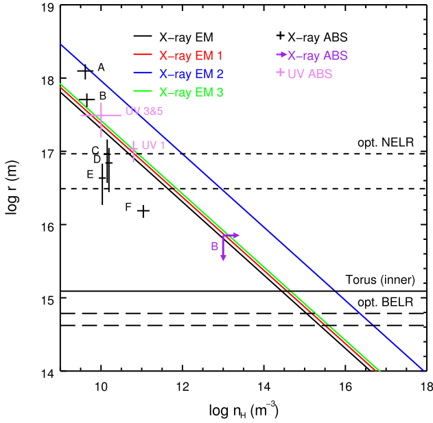
Fig. 7. Distance and number density of optical, UV and X-ray emission and/or absorption components in NGC 5548. The solid diagonal lines are the distance and density relations (i.e. \log \xi = L/n_H r^2 ) of the X-ray emission components (EM for Whewell et al. 2015, and EM 1–3 for Model T). The black pluses ( 1\sigma uncertainties) refer to the six warm absorber components (via a timing analysis, Ebrero et al. 2016). The purple arrows are the 3\sigma upper (distance) and lower (density) limits of the warm absorber component B (via a spectral analysis, Mao et al. 2017). The pink pluses are for the UV absorption components (Arav et al. 2015). The horizontal short dashed lines refer to the optical narrow emission line region (Peterson et al. 2013). The horizontal long dashed lines refer to the optical broad emission line region (Kaspi et al. 2000; Bottorff et al. 2002). The horizontal dotted line indicates the inner edge of the torus (Suganuma et al. 2006).
