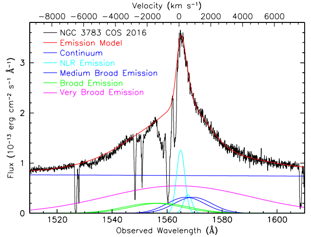
Fig. 12. Best fit with no absorption to the average COS spectrum of the C IV region from observations in 2016 December. The black histogram shows the data. The solid red line tracing the data is the total emission model. The key in the figure identifies the emission components in our model. The velocity scale along the top axis is for the blue component of the C IV doublet, \lambda 1548.195 , relative to the host galaxy systemic redshift, z = 0.00973 (Theureau et al. 1998).
