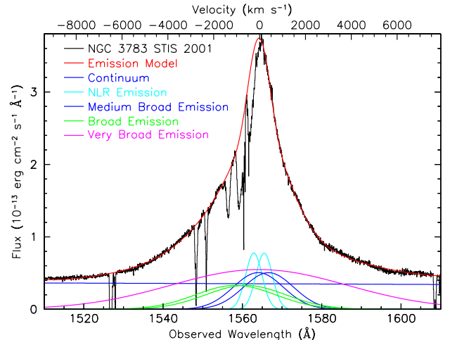
Fig. 2. Average STIS spectrum of the C iv region from all observations in the 2000–2001 campaign re-binned into 0.05 \text{ \AA} pixels (black histogram). The solid red line tracing the data shows the total emission model. The key in the figure identifies the emission components in our model. The velocity scale along the top axis is for the blue component of the C iv doublet, \lambda 1548.195 , relative to the host galaxy systemic redshift, z = 0.00973 (Theureau et al. 1998).
