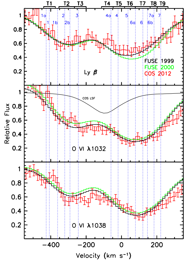
Fig. 4. Normalized spectra comparing the intrinsic absorption features in Mrk 509 from the COS G140L spectrum obtained in 2012 (red, with 1 \sigma error bars) to FUSE spectra from 1999 (black) and 2000 (green). Relative fluxes are plotted as a function of velocity relative to the host galaxy redshift of z = 0.034397 (Fisher et al. 1995). The blue dotted vertical lines are labeled with the components identified by Kriss et al. (2011) at higher spectral resolution. As a guide to the expected widths of unresolved spectral features, the COS LSF is shown as the thin black line in the middle panel. The boundaries of the selected spectral regions used to evaluate variability in the absorption troughs are indicated along the top horizontal axis (see also Table 5).
