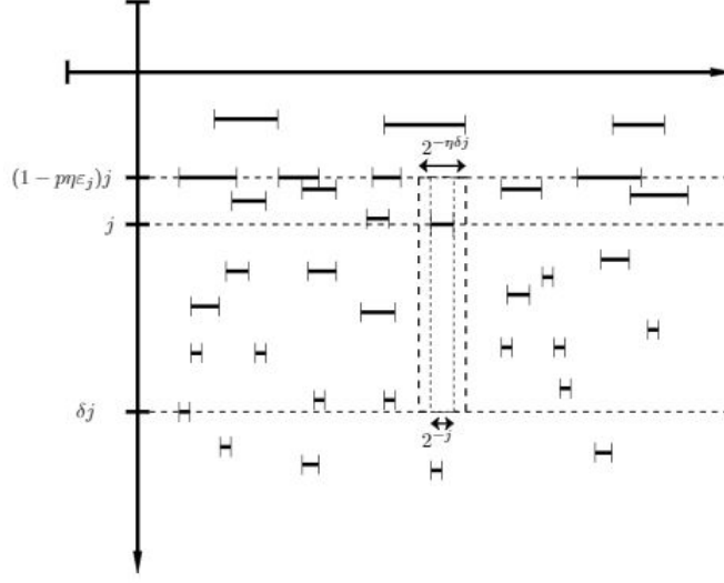
FIGURE 4. Representation of pulses supports in \mathcal{I}_j .
