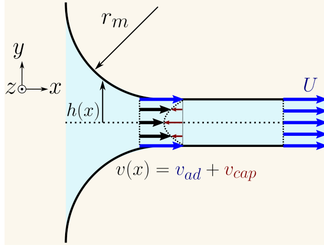
Figure 14: Notations for the Frankel problem. A flat film is connected to a meniscus along the x axis. A steady plug flow U is imposed far from the meniscus, and this latter has a constant curvature \partial_{xx}h = 1/r_m in x \rightarrow -\infty . The steady flow at the junction (called the dynamic meniscus) is the sum of an outward plug flow v_{ad} and an inward capillary flow v_{cap} .
