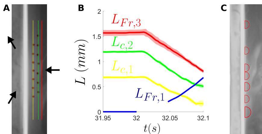
Figure 3.43: Positions of the edge of prepared Frankel film and the photobleached columns. A : Zoom near the meniscus in film 3. The vertical bright fringe on the middle left is the free meniscus, film 3 is on its right. The red line localises the detected edge of prepared Frankel film, whose distance from the edge of free meniscus is L_{Fr,3} , the green and yellow lines localise the two columns of photobleached dots, whose distances from the edge of meniscus are L_{c,1} and L_{c,2} . B : Time evolution of the distances defined in A as well as L_{Fr,1} (blue) the outgoing length of interface in film 1. The main deformation happens at t_1 = 32 s, where film 3 is compressed and film 1 is stretched. C : Towards the end of the deformation, the marginal regeneration instability appears, breaking our invariance by translation and thus stopping the measurement of the exchanged quantities of interface.
