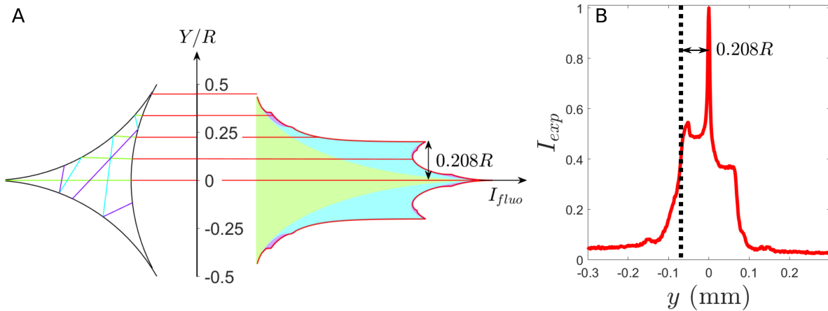
Figure 3.21: Ray tracing simulation for a fluorescent meniscus. A: we define an ideal free meniscus composed of three interfaces of curvatures R in contact. The red lines are the outgoing rays seen by the side. On the right, the resulting intensity profile as a function of the ordinate (normalised by R ), where the shaded coloured areas are the contributions of the different rays: ray without reflection (green), with one reflection (light blue), or two reflections (purple). B: Identification of the intensity drop on experimental data.
