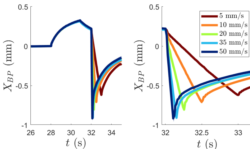
Figure 3.29: Horizontal displacement of the free meniscus throughout the whole “Push 3” experiment, for [DOH] = 50\ \text{mg/L} and a varying velocity of main deformation V_1 . The figure on the right is just a zoom around t_1 = 32\ \text{s} of the figure on the left. At t_0 = 28\ \text{s} , the horizontal film 3 is prepared, meaning it is being stretched at V_0 = 2\ \text{mm/s} from 4.2\ \text{mm} to 10\ \text{mm} , leading to a first displacement of the free meniscus in +x . At t_1 = 32\ \text{s} , the main deformation of the “Push 3” experiment is performed at V_1 varying between 5 - 50\ \text{mm/s} .
