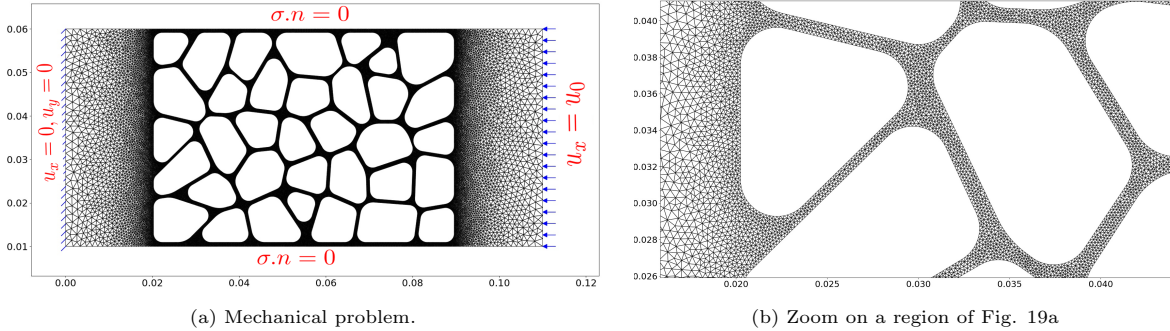
Figure 19: Virtual finite element test.
