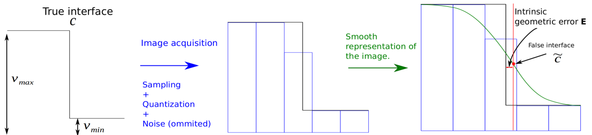
Figure 6: Steps for constructing the synthetic image and the use of a smooth representation of the image.
