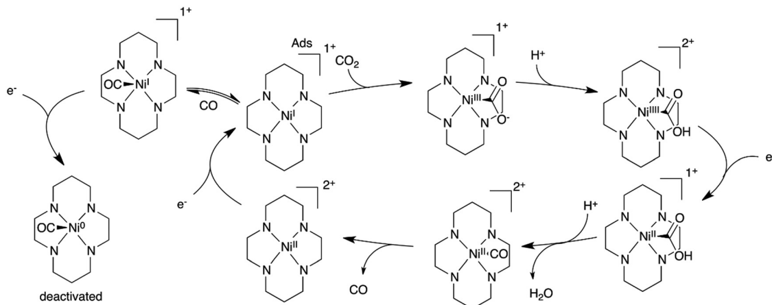
Scheme 1 Proposed electrochemical reduction mechanism of \text{CO}_2 to \text{CO} in water with the Ni1 catalyst adsorbed at a Hg electrode.
