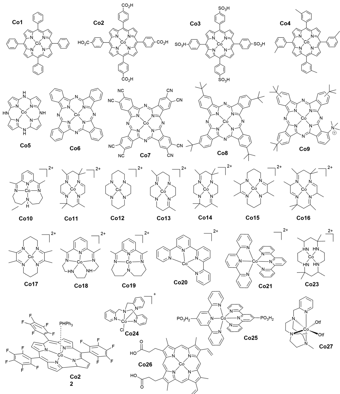
Chart 1 Cobalt complexes.
