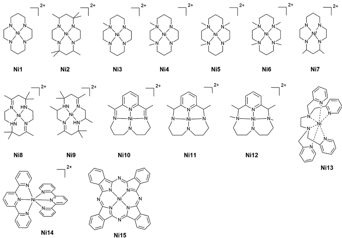
Chart 2 Nickel complexes.
